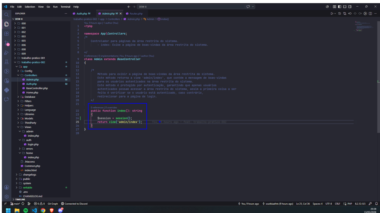
Figura 5 - Admin::index
