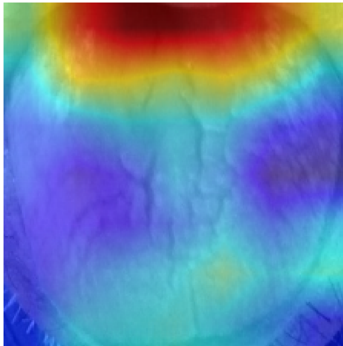
Baseline (ResNet101)
