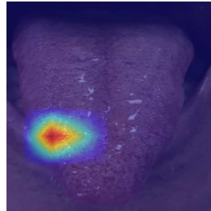
Ours (Proposed)
