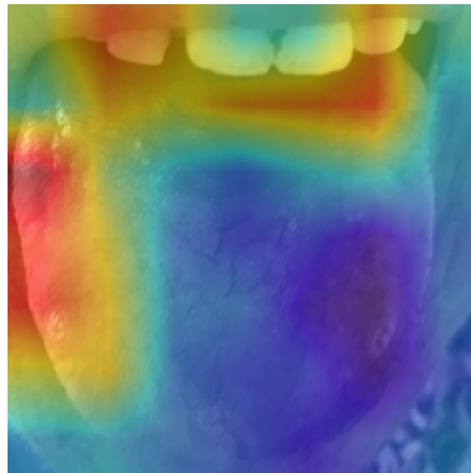
Baseline (ResNet101)
