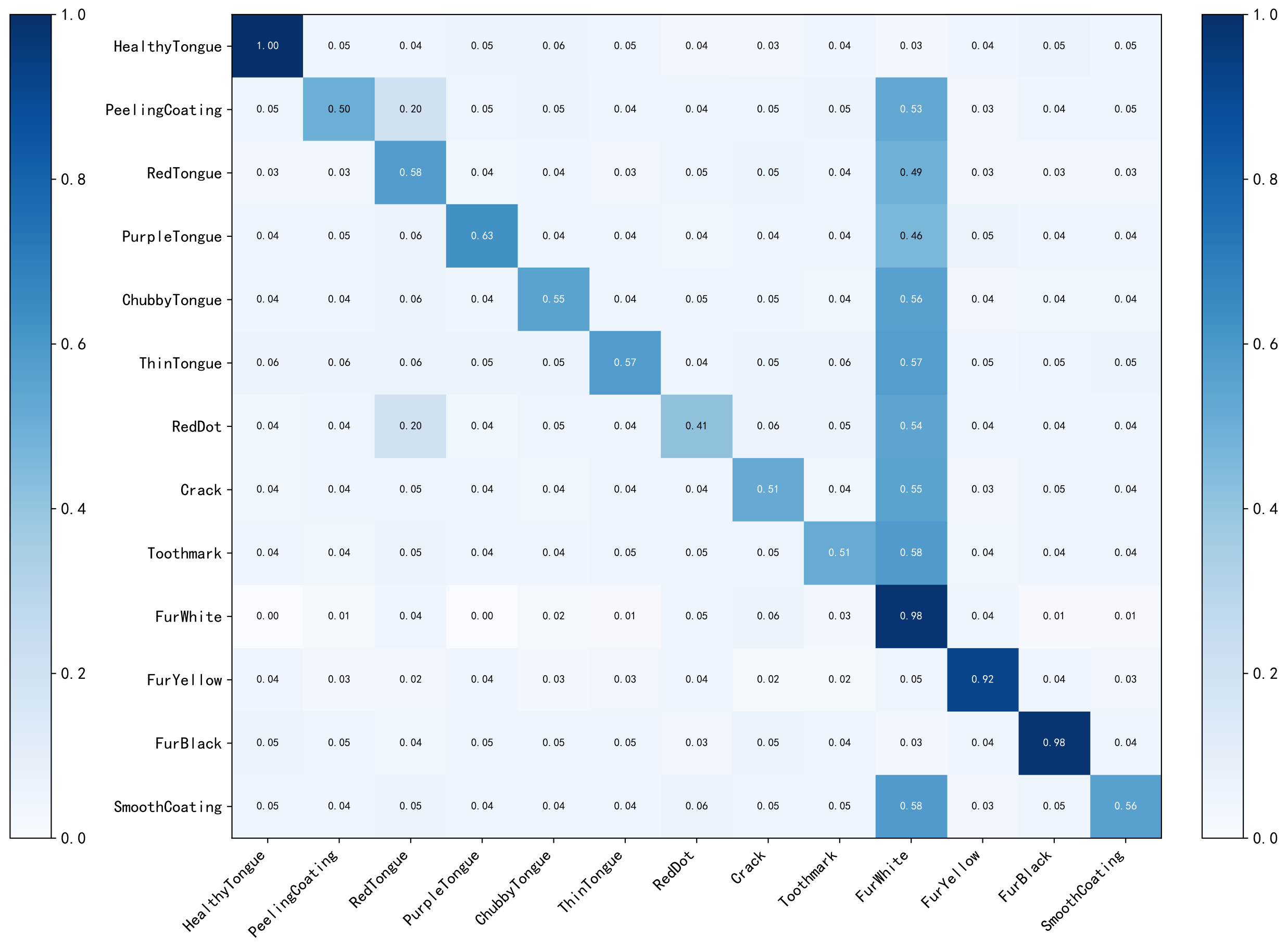
ITDD – Learned Matrix M
