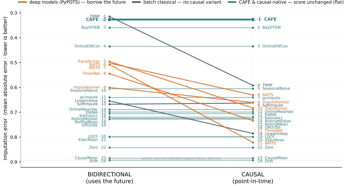
Figure 2: Forbid the future and the board collapses. Each line is a method; the y -axis is MAE on a shared scale, so a method whose score is unchanged by the protocol (every causal-native method, \Delta = 0 ) is a perfectly horizontal line, while methods that borrow from the future slope. Left = bidirectional MAE (the standard game), right = causal (strict point-in-time) MAE, averaged over the structured real datasets (FX excluded as a no-structure control). The methods that win bidirectionally by reading the future (linear interpolation, TRMF, the deep imputers) cannot compete causally and slope up or drop off; CAFÉ is flat (it borrows nothing, \Delta = 0 ) and rises to #1 on the causal side even though TRMF edges it bidirectionally by reading the future. The causal column is the only one valid for a backtest.
