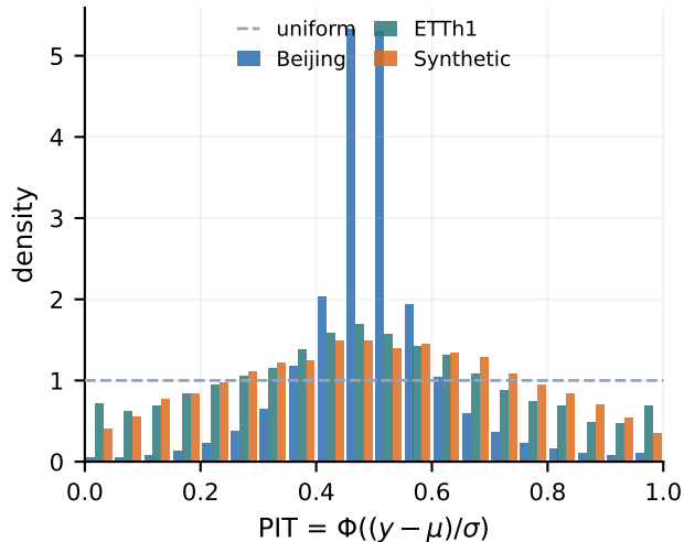
(b) PIT histogram (flat = calibrated)
