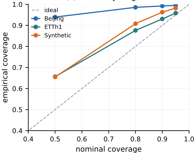
(a) Reliability diagram
