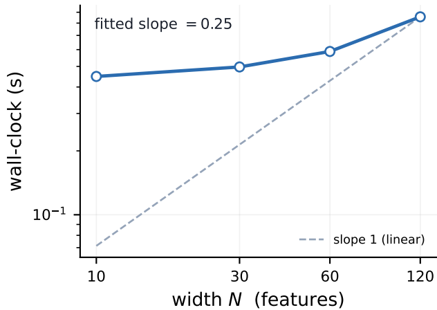
CAFÉ vs N (fixed T = 2000 )
