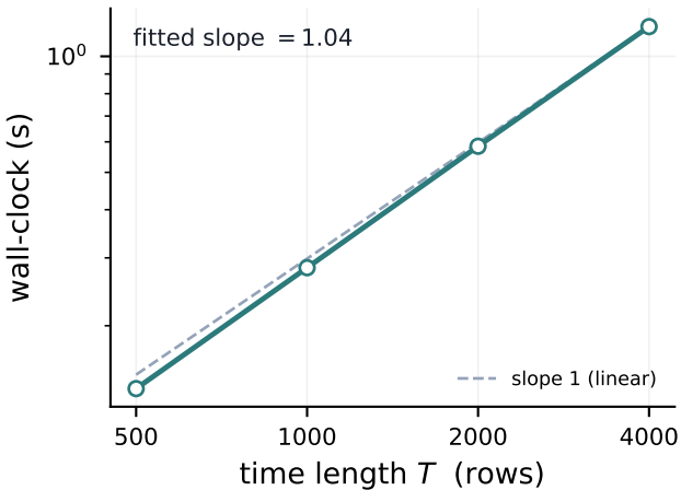
CAFÉ vs T (fixed N = 60 )
