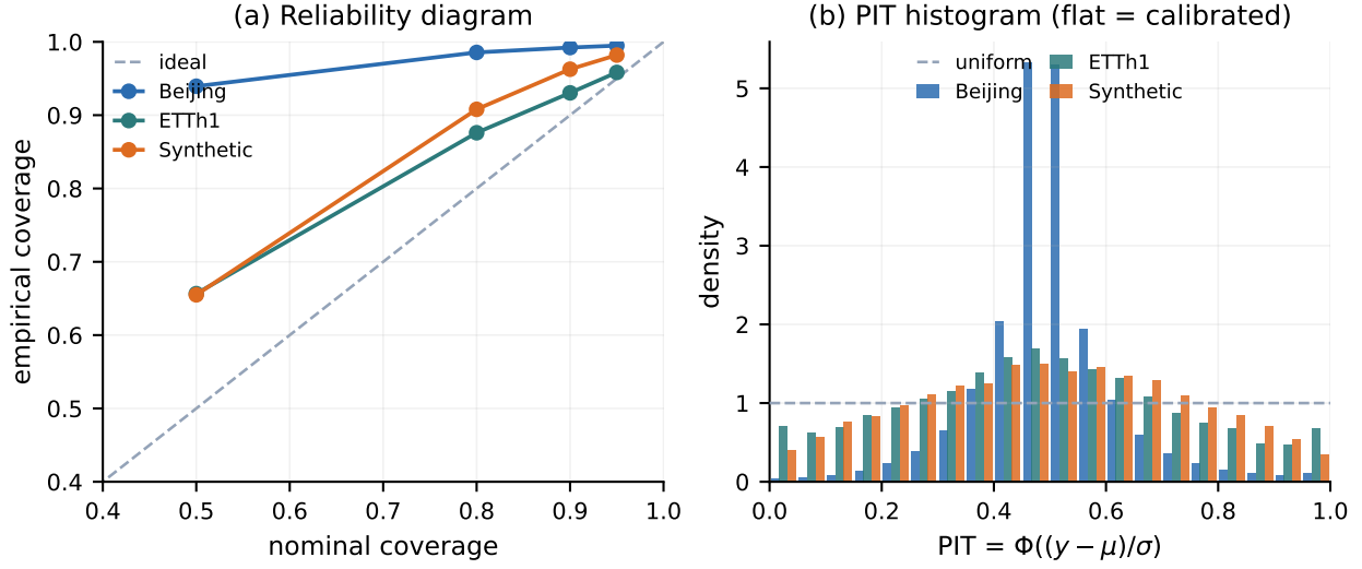
Figure 14: Calibration (Table 9) . (a) Reliability diagram: empirical vs. nominal coverage—every curve sits on or above the diagonal, so CAFÉ never under-covers. (b) PIT histograms: a flat profile would be sharply calibrated; CAFÉ’s are centre-peaked, the signature of conservative (over-dispersed) intervals—safe, but loose, on the smoother panels.
