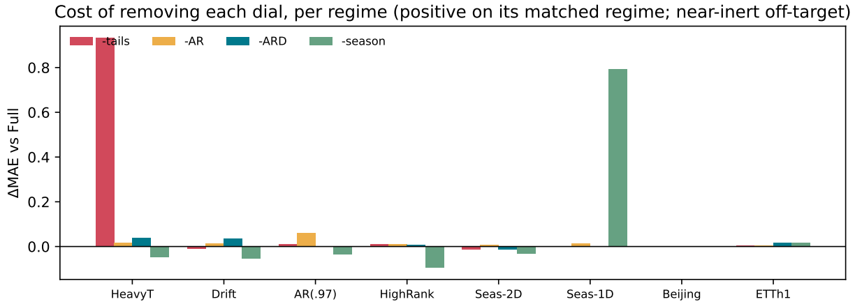
Figure 15: Full ablation matrix (Table 6) . Cost of removing each dial ( \Delta\text{MAE} vs. full CAFÉ) across all eight regimes. Each dial spikes on the regime it targets and is near-inert—small, often slightly negative—elsewhere, the price of empirical-Bayes priors that shrink an unsupported dial toward off rather than exactly to it.
