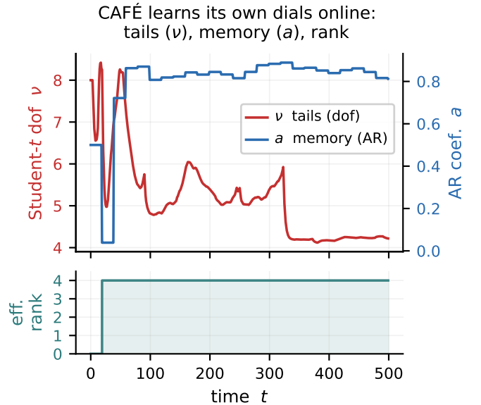
Figure 8: Self-tuning dials. The tails ( \nu ), memory ( a ) and effective rank adapt online from the data—no hyper-parameters.
