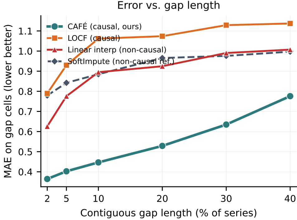
Figure 13: Graceful degradation under long gaps (Table 14) . Imputation MAE as a single contiguous gap grows to 40% of the series. Local causal methods (LOCF, linear) saturate near the unconditional error; CAFÉ stays bounded and beats even the non-causal SoftImpute reference at every length.
