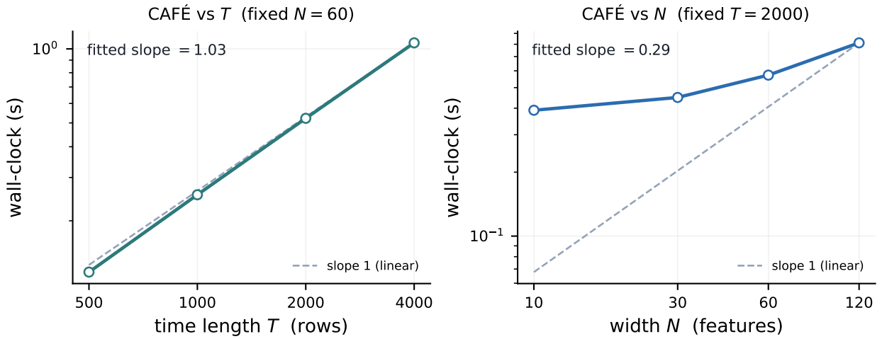
Figure 14: Scaling (Table 18) . Wall-clock vs. series length T (near-linear, log-log slope \approx 1 ) and vs. width N (strongly sub-linear): each row uses only rank- R Cholesky solves, never an N \times N inverse.
