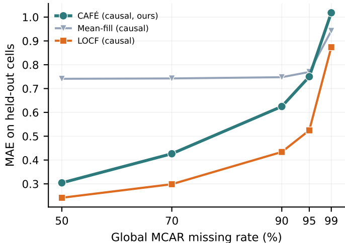
(a) Degradation to 99% missing (real panels: Beijing/ETTh1/FRED-MD)
