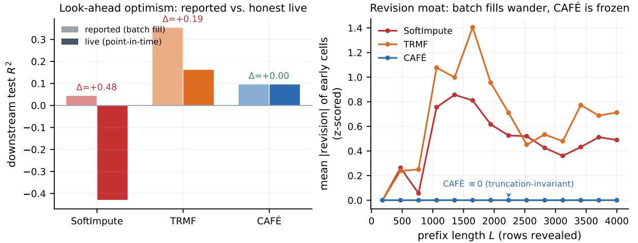
Figure 11: The cost of look-ahead (Table 7). Left: a downstream ridge forecaster’s reported vs. honest live R^2 on ETTh1; batch (bidirectional) imputation inflates the reported score, and the same fixed model is worse live, while CAFÉ is identical both ways. Right: mean |revision| of an early imputed cell as the future is revealed—batch methods keep rewriting their own past, CAFÉ is flat at zero.
