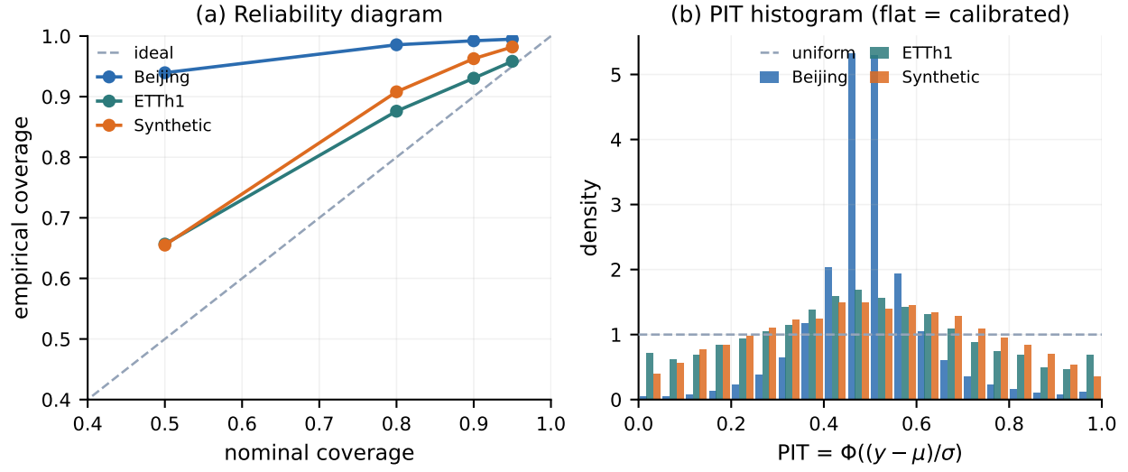
Figure 14: Calibration (Tables 14, 15). (a) Reliability diagram: empirical vs. nominal coverage—curves sit on or above the diagonal at most levels (predominantly over-covering), with only marginal undershoots at the tightest levels. (b) PIT histograms: a flat profile would be sharply calibrated; CAFÉ’s are centre-peaked, the signature of conservative (over-dispersed) intervals—safe, but loose, on the smoother panels.
