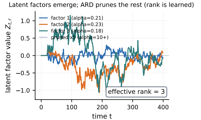
Figure 5: Latent factors & learned rank. The common factors z_t (a streaming robust DFM); ARD prunes the rest, so the effective rank is discovered, not set.
