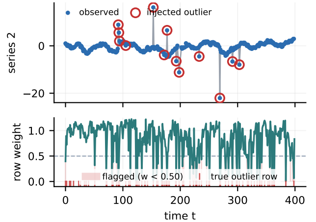
Figure 7: Anomaly detection (free). The Student- t weights drop exactly on injected outliers—a point-in-time data-quality / fault score from the same pass.
