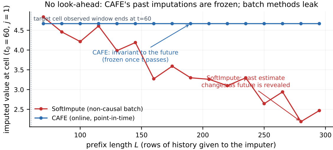
Figure 2: The moat: no look-ahead. For a fixed early missing cell, we re-impute on growing time-prefixes. CAFÉ’s estimate is frozen the moment its time passes (flat line), so a backtest cannot be contaminated; the non-causal batch method’s “past” estimate keeps changing as the future is revealed. This is what makes CAFÉ safe for sequential decision-making.
