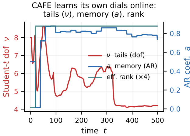
Figure 8: Self-tuning dials. The tails ( \nu ), memory ( a ) and effective rank adapt online from the data—no hyper-parameters.
