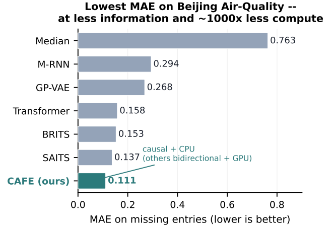
Figure 10: Accuracy. Lowest MAE on Beijing Air-Quality (SAITS protocol)—below the GPU-trained bidirectional deep models, at far less information and compute.
