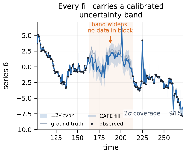
Figure 4: Calibrated uncertainty. Every fill carries a posterior band that widens inside long gaps (less information). Enables confidence intervals, error propagation, and multiple imputation.
