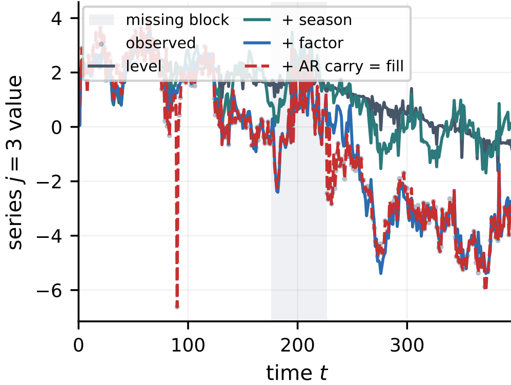
Figure 3: Interpretability. The imputed value is the sum of human-readable parts—level, season, shared factors, idiosyncratic carry—read from the trace, not a black box. Each term can be inspected, audited, or used on its own.
