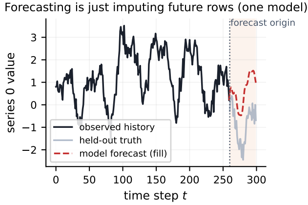
Figure 9: Forecasting = imputation. Masking the last rows and imputing them yields a forecast via the AR/Kalman state—one model for fill, forecast and now-cast.
