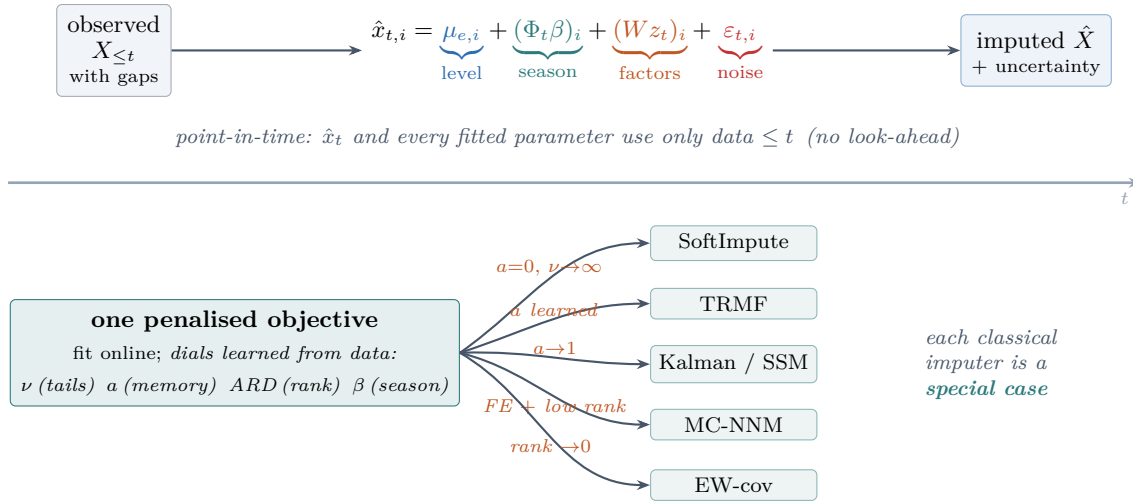
Figure 1: CAFÉ in one picture. Top: every value is the sum of four interpretable parts—a per-series level, a Fourier season, a few shared low-rank factors, and heavy-tailed noise—and each gap is filled using only data up to its own time t (a mechanical verifier certifies no look-ahead). Bottom: a single penalised objective whose dials (Student- t \nu , AR a , ARD rank, seasonal \beta ) are learned from the data; classical imputers are the corners of this parameter space, so there is no model to select.
