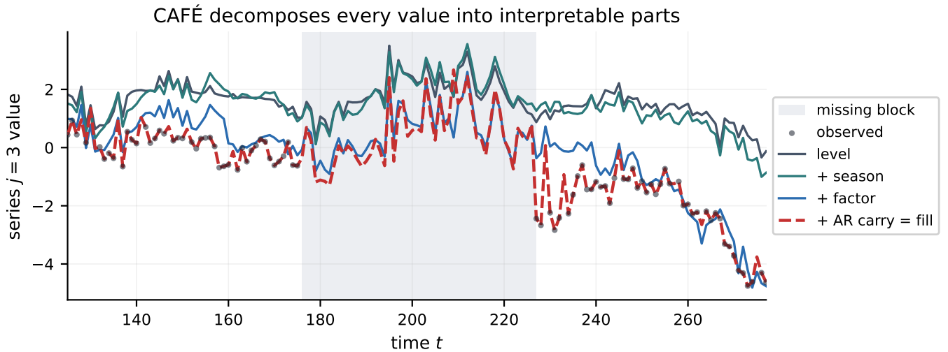
Figure 5: Interpretability. The imputed value is the sum of human-readable parts—level, season, shared factors, idiosyncratic carry—read from the trace, not a black box. Each term can be inspected, audited, or used on its own.
