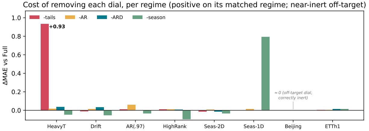
Figure 18: Full ablation matrix (Table 16). Cost of removing each dial ( \Delta\text{MAE} vs. full CAFÉ) across all eight regimes. Each dial spikes on the regime it targets and is near-inert—small, often slightly negative—elsewhere, the price of empirical-Bayes priors that shrink an unsupported dial toward off rather than exactly to it.
