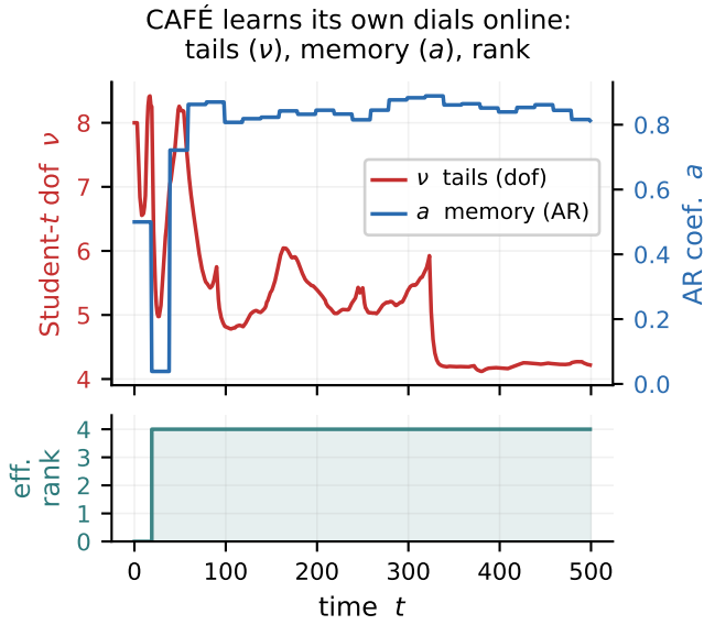
Figure 10: Self-tuning dials. The tails ( \nu ), memory ( a ) and effective rank adapt online from the data—no hyperparameters.
