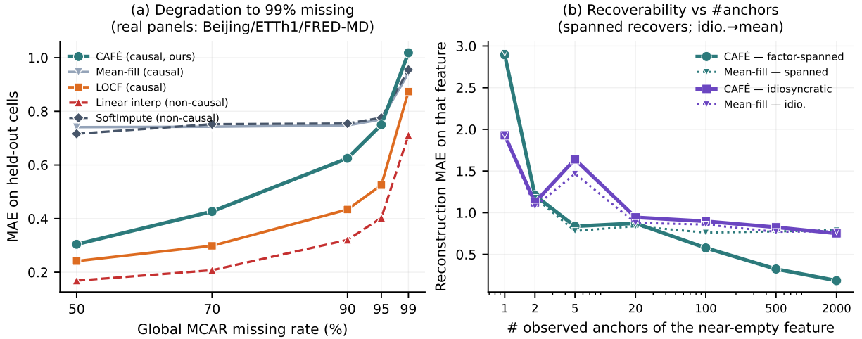
Figure 16: Extreme missingness and the recoverability frontier (Table 19). Left : MAE under global MCAR up to 99%—CAFÉ stays finite and beats the naive causal fills. Right : reconstruction MAE of a single near-empty feature vs. the number of observed anchors k : when the feature is factor-spanned CAFÉ recovers it (margin over mean-fill grows with k ), when it is idiosyncratic CAFÉ tracks the mean rather than hallucinating; k \leq 2 is the honest identifiability floor.
