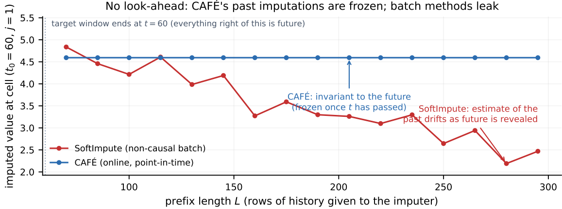
Figure 4: The moat: no look-ahead. For a fixed early missing cell, we re-impute on growing time-prefixes. CAFÉ’s estimate is frozen the moment its time passes (flat line), so a backtest cannot be contaminated; the non-causal batch method’s “past” estimate keeps changing as the future is revealed. This is what makes CAFÉ safe for sequential decision-making.
