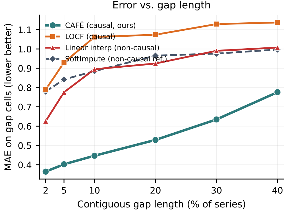
Figure 13: Graceful degradation under long gaps (Table 18) . Imputation MAE as a single contiguous gap grows to 40% of the series. Local causal methods (LOCF, linear) saturate near the unconditional error; CAFÉ stays bounded and beats even the non-causal SoftImpute reference at every length.
