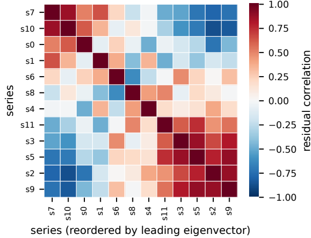
Figure 8: Dependency network. The residual covariance recovers the cross-sectional correlation structure between series—useful as features and for contagion analysis.
