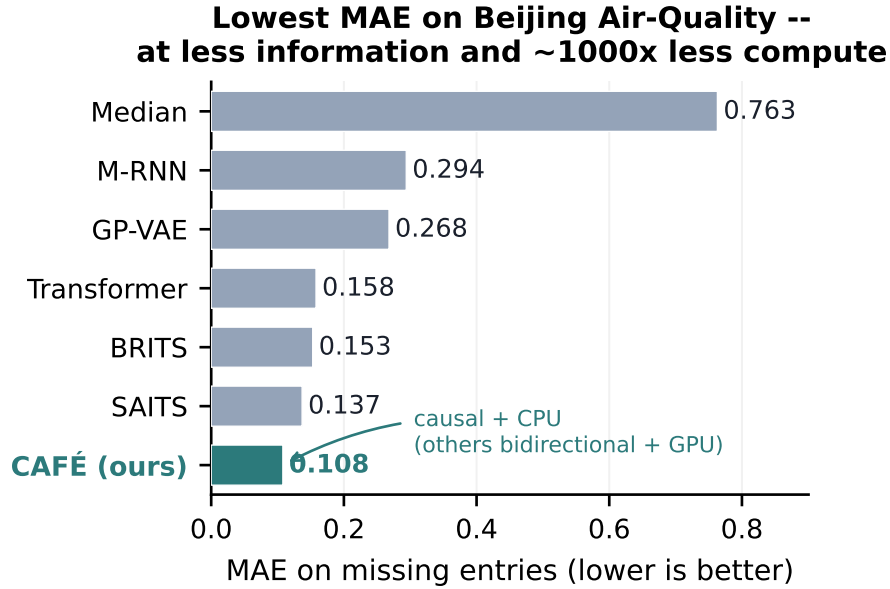
Figure 12: Accuracy. CAFÉ’s MAE on the named Beijing Air-Quality slice (10% point/MCAR, standardised, 3 seeds) lands in the band of GPU-trained bidirectional deep models—at far less information and compute, and while remaining causal. Published deep numbers (different protocols) are context, not a head-to-head ranking; see Table 8.
