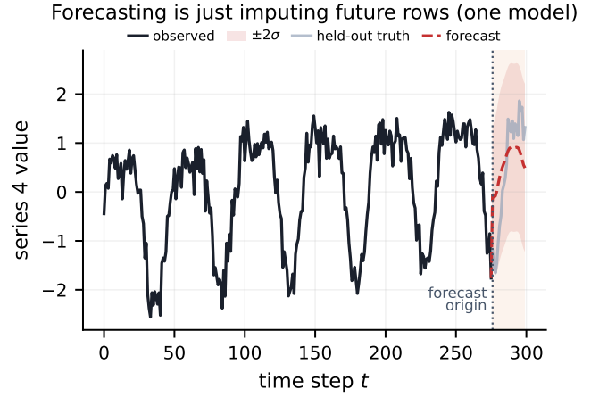
Figure 11: Forecasting = imputation. Masking the last rows and imputing them yields a forecast via the AR/Kalman state—one model for fill, forecast and now-cast. The shaded \pm 2\sigma cone is the model’s own predictive variance, widening with horizon as the latent state’s information decays.
