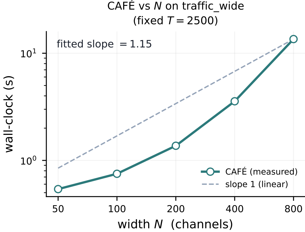
Figure 15: Scaling at real width (Table 25). Wall-clock vs. width N on the full 862-sensor Traffic panel (a decade wider than the race panels): the measured log-log slope is \approx 1.15 , confirming CAFÉ stays near-linear in N at scale.
