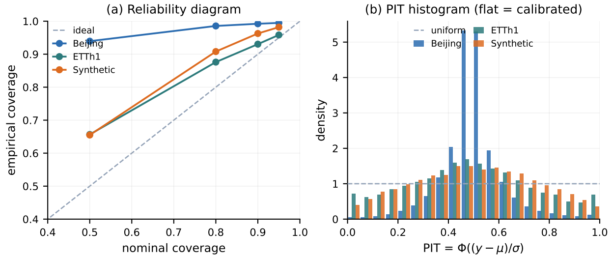
Figure 17: Calibration (Table 21). (a) Reliability diagram: empirical vs. nominal coverage—curves sit on or above the diagonal at most levels (predominantly over-covering), with only marginal undershoots at the tightest levels. (b) PIT histograms: a flat profile would be sharply calibrated; CAFÉ’s are centre-peaked, the signature of conservative (over-dispersed) intervals—safe, but loose, on the smoother panels.
