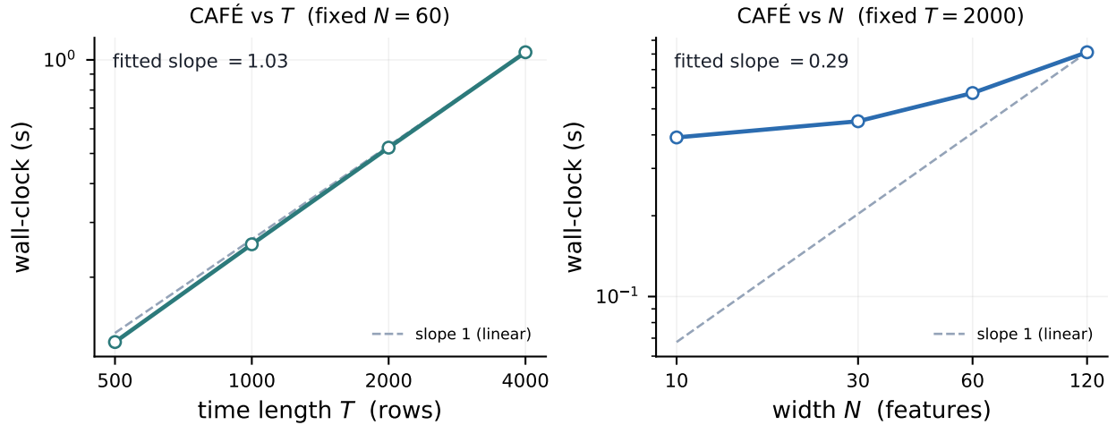
Figure 14: Scaling (Table 24) . Wall-clock vs. series length T (near-linear, log-log slope \approx 1 ) and vs. width N (strongly sub-linear): each row uses only rank- R Cholesky solves, never an N \times N inverse.
