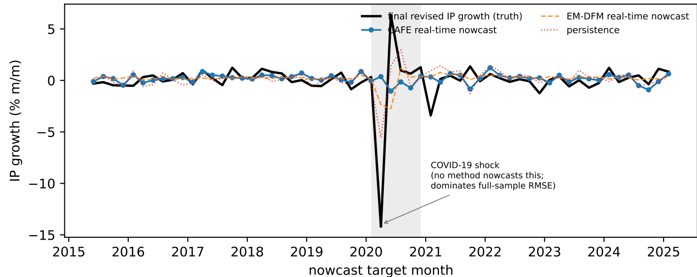
Real-time nowcasts vs final revised industrial production
