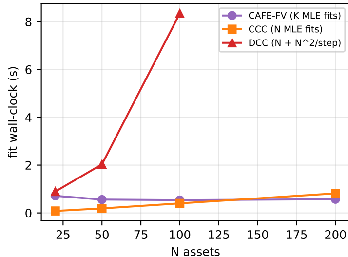
(c) Runtime: CAFE-FV flat in N, DCC super-linear / infeasible
