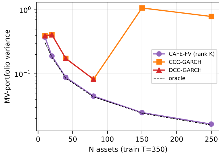
(a) Curse of dimensionality: DCC/CCC blow up, CAFE-FV improves
