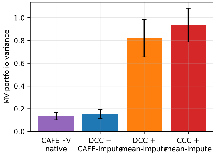
(b) 16% async gaps: native CAFE-FV wins; naive impute is catastrophic
