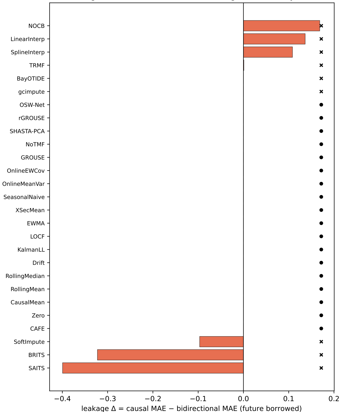
Leakage leaderboard: certified causal (green) vs leaky (red)
