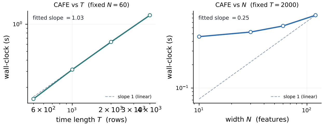
Figure 13: Scaling (Table 9) . Wall-clock vs. series length T (log-log slope 1.03, near-linear) and vs. width N (slope 0.25, sub-linear): each row uses only rank- R Cholesky solves, never an N \times N inverse.
