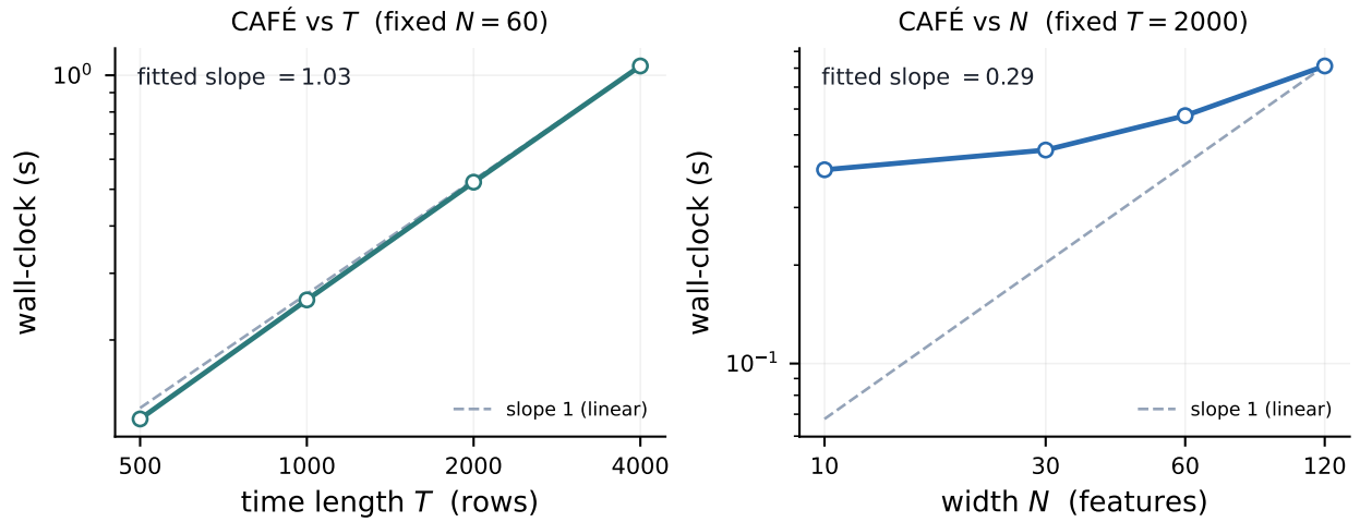
Figure 13: Scaling (Table 15). Wall-clock vs. series length T (near-linear, log-log slope \approx 1 ) and vs. width N (strongly sub-linear): each row uses only rank- R Cholesky solves, never an N \times N inverse.
