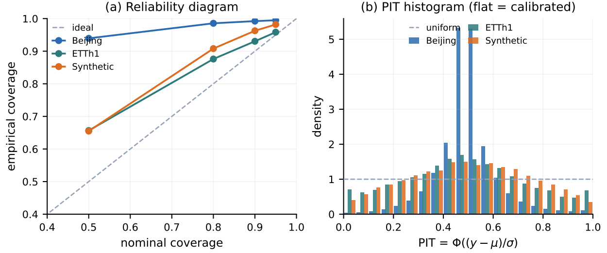
Figure 14: Calibration (Table 14). (a) Reliability diagram: empirical vs. nominal coverage—curves sit on or above the diagonal at most levels (predominantly over-covering), with only marginal undershoots at the tightest levels. (b) PIT histograms: a flat profile would be sharply calibrated; CAFÉ’s are centre-peaked, the signature of conservative (over-dispersed) intervals—safe, but loose, on the smoother panels.
