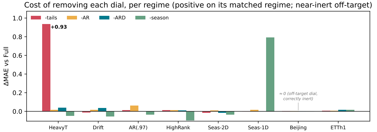
Figure 15: Full ablation matrix (Table 10). Cost of removing each dial ( \Delta MAE vs. full CAFÉ) across all eight regimes. Each dial spikes on the regime it targets and is near-inert—small, often slightly negative—elsewhere, the price of empirical-Bayes priors that shrink an unsupported dial toward off rather than exactly to it.
