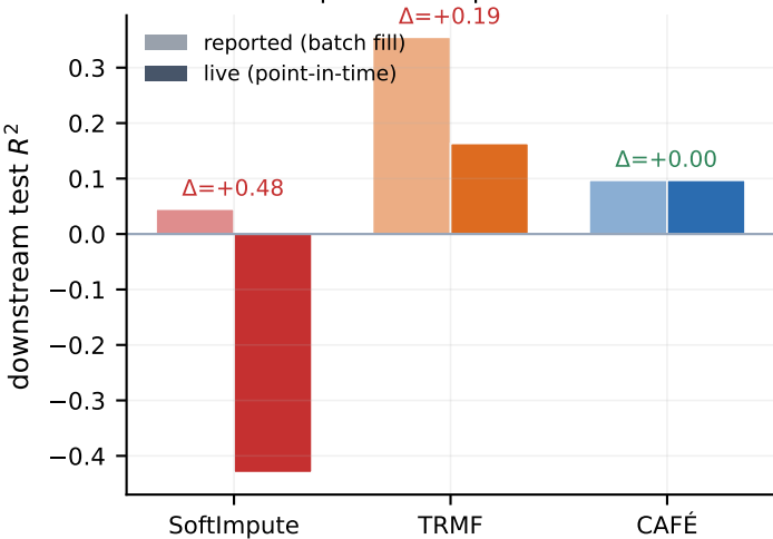
Look-ahead optimism: reported vs. honest live
