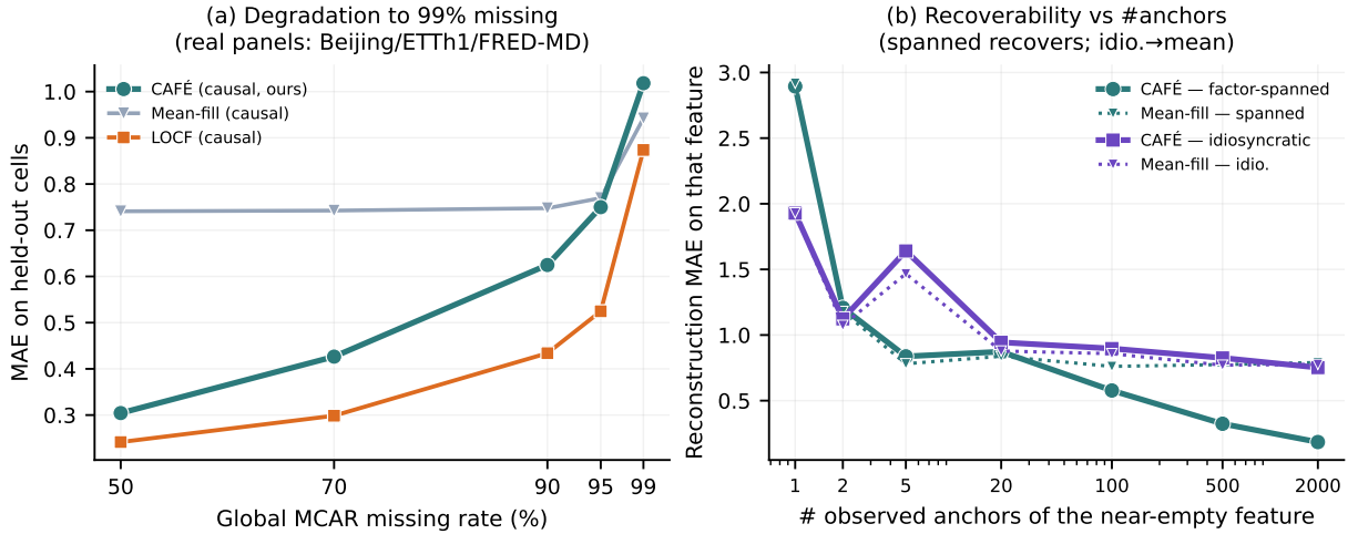
Figure 21: Extreme missingness and the recoverability frontier (Table 25). Left : MAE under global MCAR up to 99% (causal methods only)—CAFÉ stays finite and bounded below mean-fill, while carry-forward (LOCF) wins under scattered point missingness. Right : reconstruction MAE of a single near-empty feature vs. the number of observed anchors k : when the feature is factor-spanned CAFÉ recovers it (margin over mean-fill grows with k ), when it is idiosyncratic CAFÉ tracks the mean rather than hallucinating; k \leq 2 is the honest identifiability floor.
