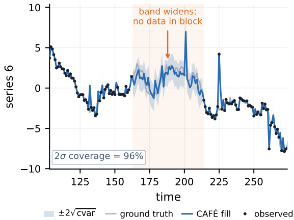
Figure 11: Conservative uncertainty. Every fill carries a posterior band that widens inside long gaps (less information). The bands are predominantly over-conservative —they over-cover at most levels (a safe failure mode for decision-making), with only marginal undershoots at the tightest levels—and enable confidence intervals, error propagation, and multiple imputation. Scored by CRPS / coverage / sharpness (Table 28).
