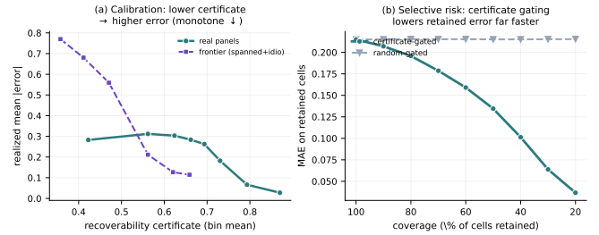
Figure 8: Selective imputation via the recoverability certificate. (a) Calibration: mean held-out [error] falls monotonically as the certificate rises. (b) Risk-coverage: abstaining on the least-confident cells (certificate-gated) drops retained MAE far faster than random abstention.
