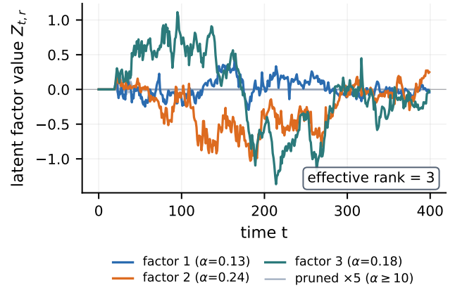
Figure 12: Latent factors & learned rank. The common factors z_t (a streaming robust DFM); ARD prunes the rest, so the effective rank is discovered, not set.
