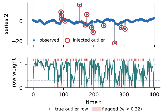
Figure 14: Anomaly detection (free). The Student- t weights drop exactly on injected outliers—a point-in-time data-quality / fault score from the same pass.
