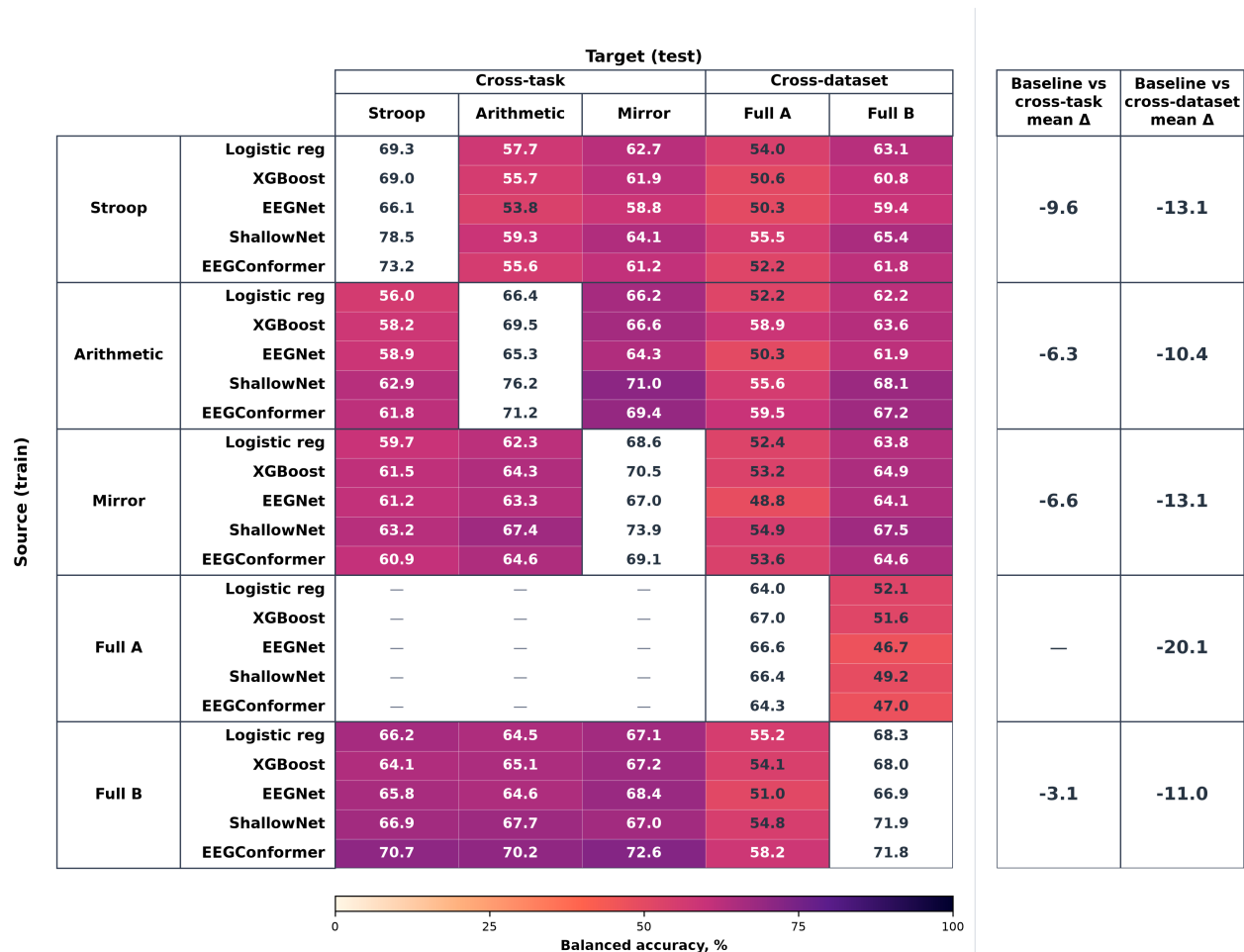
Fig 1. Zero-shot transfer performance across source and target compositions. Rows and columns denote source and target compositions. The grey diagonal shows the target-specific baseline scenario. The two right-hand columns show mean differences from the relevant target baselines; negative values indicate lower performance, and dashes mark contrasts that are not applicable.
