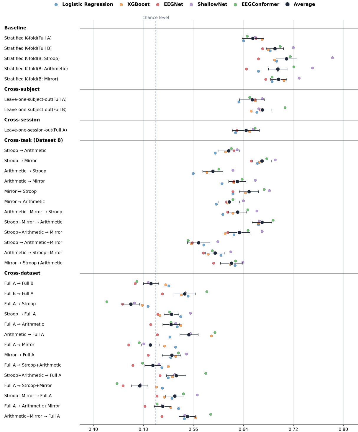
Fig 1. Balanced accuracy across experimental scenarios for the five decoders. Colored points show the individual decoders; black points and 95% bootstrap intervals show their mean.
