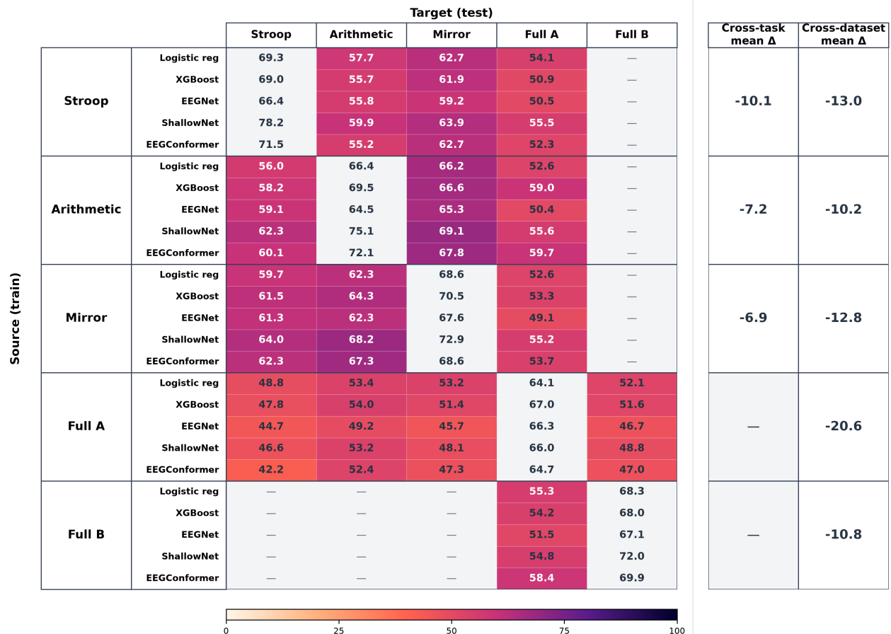
Fig 2. Zero-shot transfer performance across source and target compositions. Each cell reports balanced accuracy (%) for one decoder trained on the source composition (rows) and evaluated on the target composition (columns). Grey diagonal cells show the corresponding within-composition baselines; coloured cells show cross-task or cross-dataset transfer; dashes indicate unavailable source–target combinations. Summary columns report the mean difference in balanced accuracy relative to the target-specific baseline, averaged across decoders and compatible target compositions; negative values indicate lower transfer performance.
