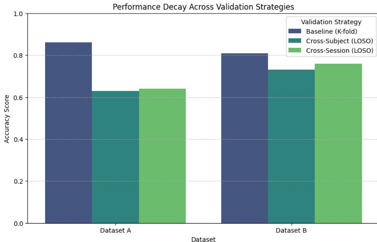
Fig 1. Performance decay across validation strategies. Classification performance decreases as the validation protocol moves from within-dataset evaluation toward cross-subject, cross-session, cross-task, and cross-dataset transfer.
