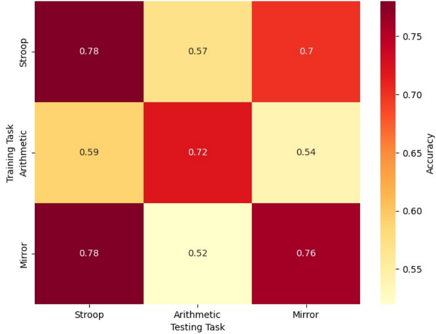
Fig 2. Cross-task generalization matrix. Pairwise transfer performance between the cognitive tasks of Dataset B (Stroop, Arithmetic, and Mirror recognition).
