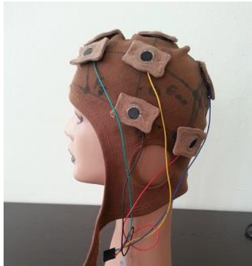
Figure 2. The modified headset
