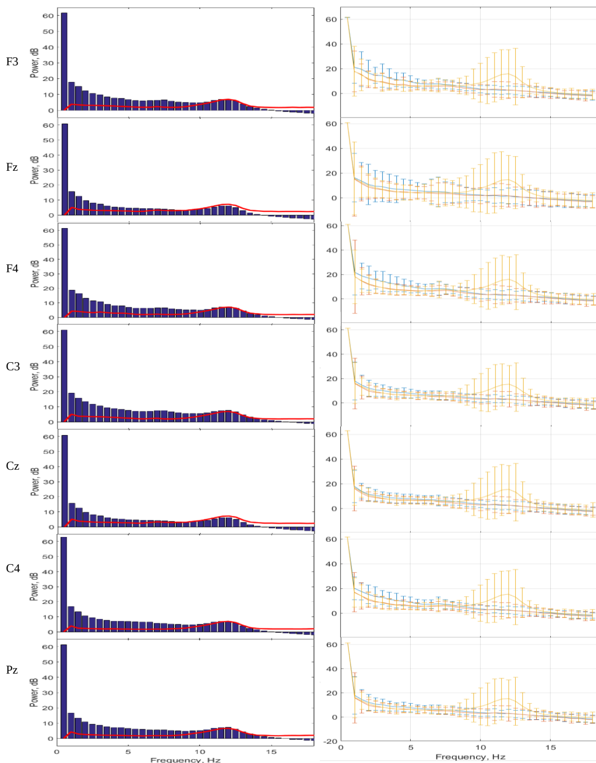
Figure 9. Examples of the feature and their basic statistical properties for participant S1.
