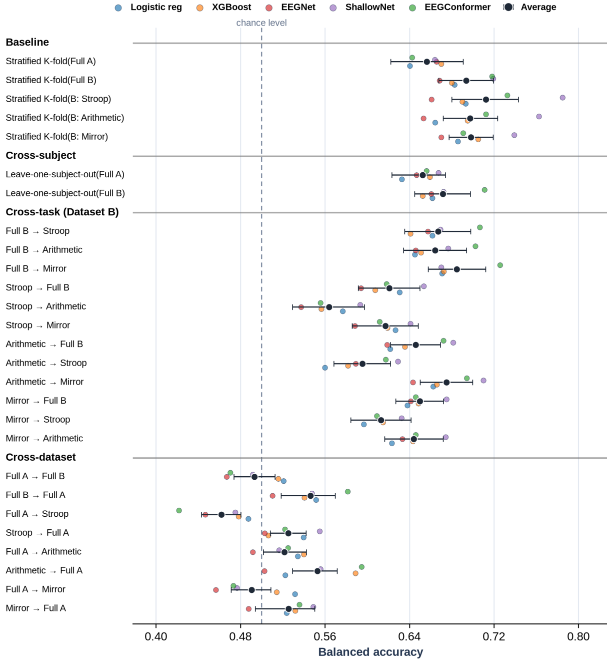
Fig 3. Participant-level balanced accuracy across experimental scenarios for the five decoders.
