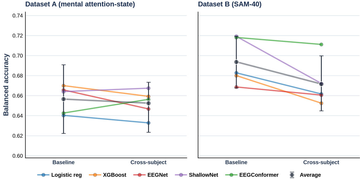
Fig 2. Baseline and cross-subject performance across decoders.
