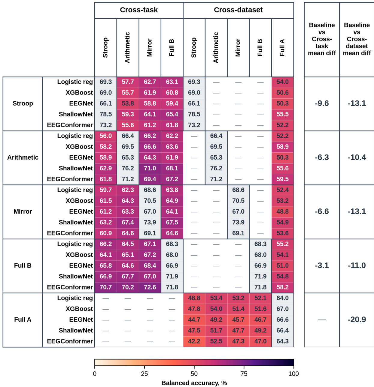
Fig 1. Zero-shot transfer performance across source and target compositions. Rows denote a decoder and the composition it was trained on, and columns denote the composition it was tested on. The gray diagonal is not a transfer but the baseline validation scenario, where a decoder was trained and tested on the same composition. The two right-hand columns show mean differences from the relevant target baselines. Negative values indicate lower performance, and dashes mark contrasts that are not applicable.
