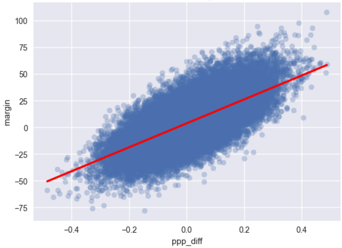
Margin vs ppp_diff
