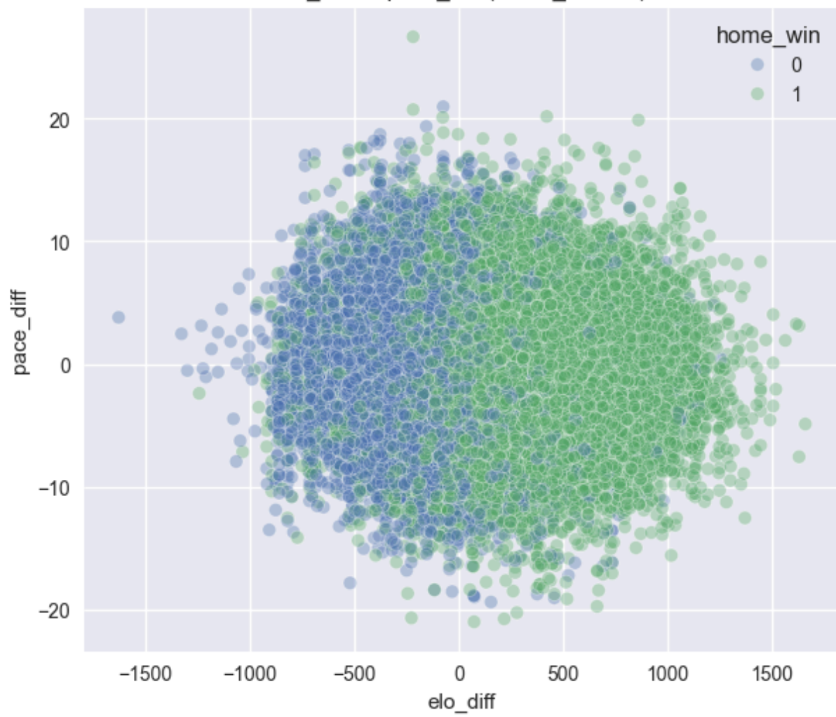
elo_diff vs pace_diff (home_win 0/1)
