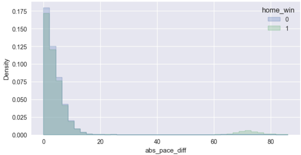
abs_pace_diff Distribution by Home Win
