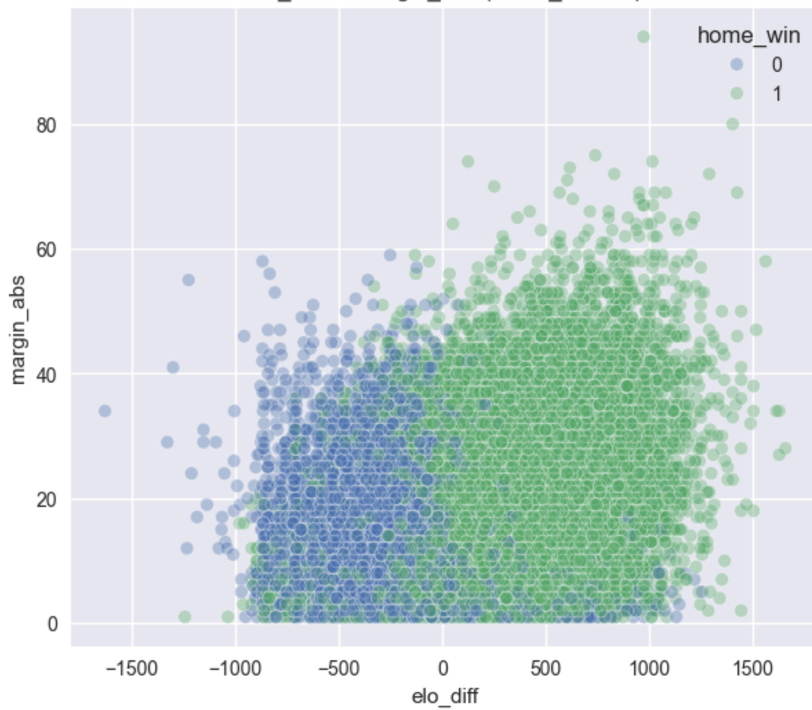
elo_diff vs margin_abs (home_win 0/1)
