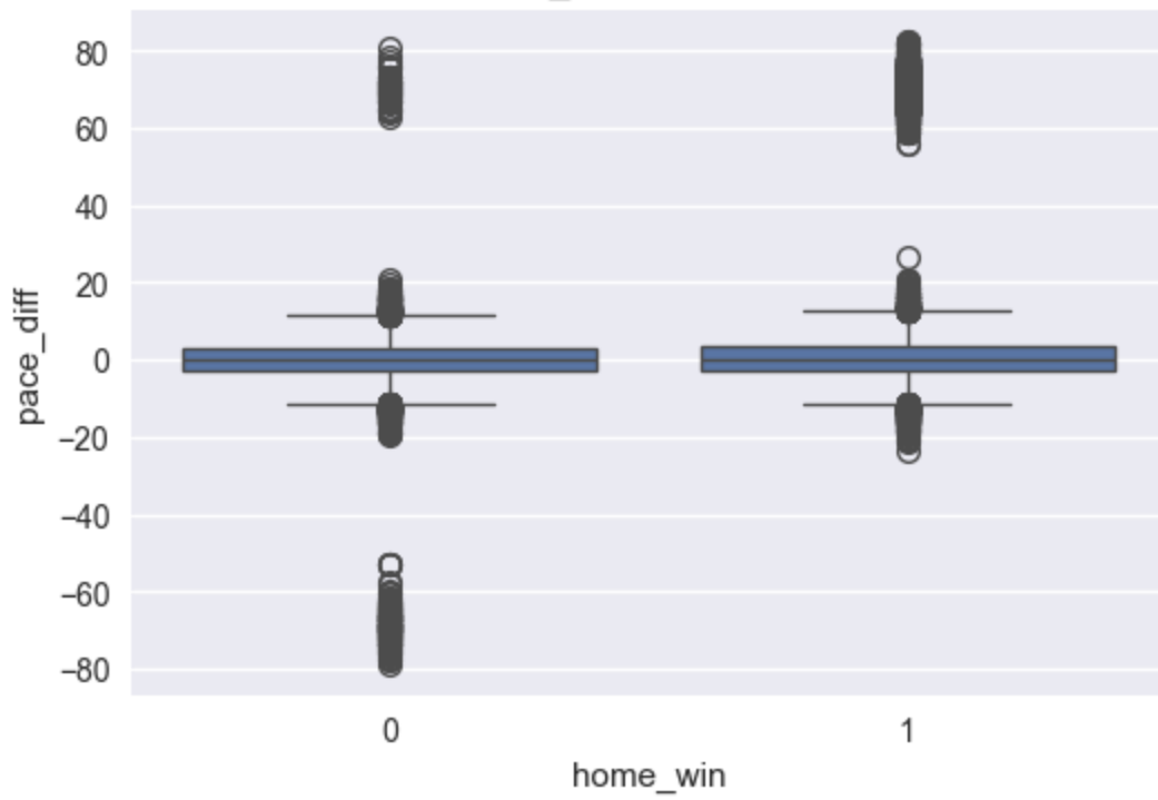
pace_diff vs Outcome
