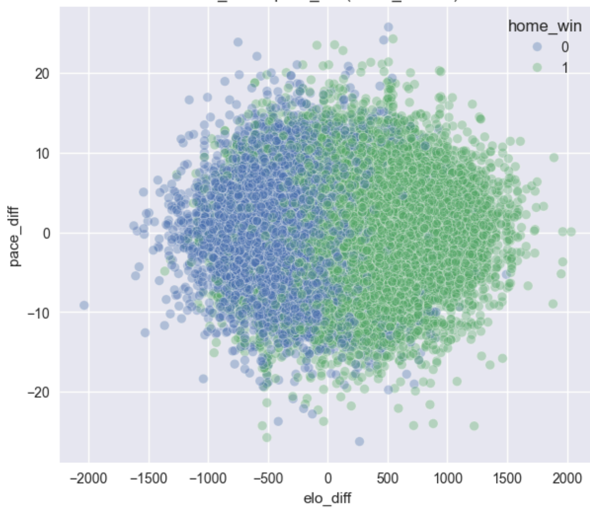
elo_diff vs pace_diff (home_win 0/1)
