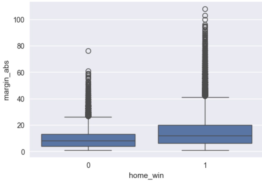
margin_abs vs Outcome
