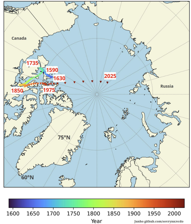
Geomagnetic North Pole Wander (1590-2025)
