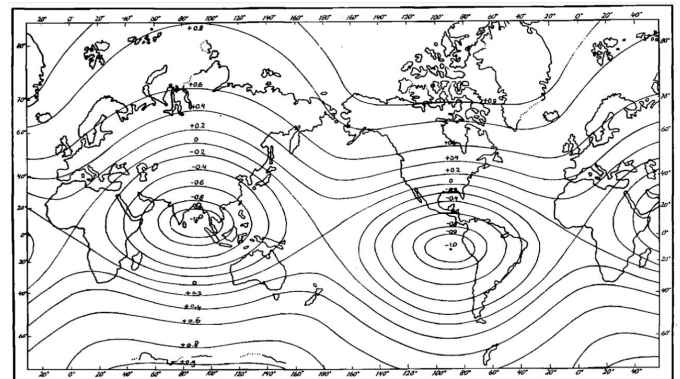
Fig. 22--World map of values of (\sigma_B + \sigma_\alpha)
