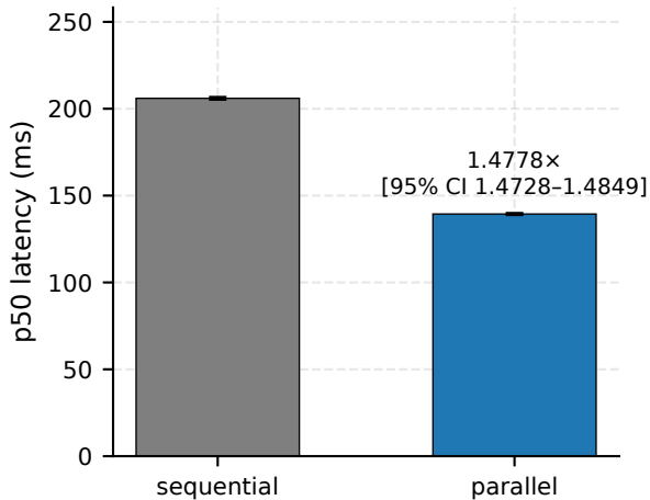
customer_support_100
