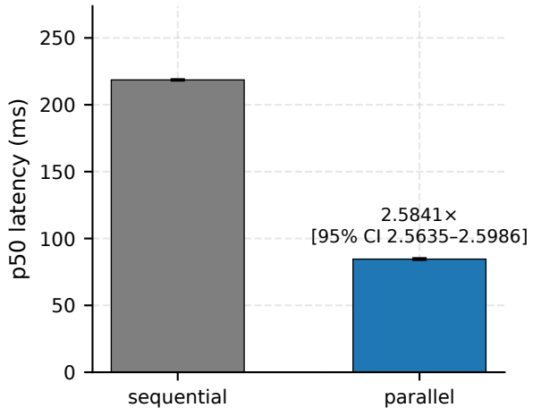
document_analysis_50
