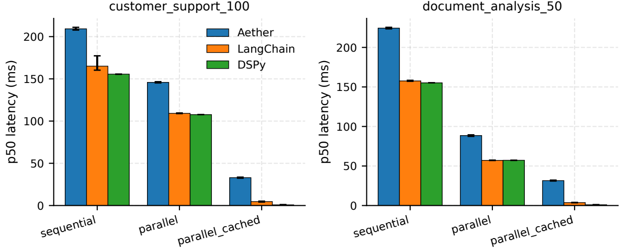
Figure 1: Per-config p50 latency (ms) across systems on synthetic mock-LLM benchmarks. Error bars are 95% paired BCa intervals. n=5 trials per config. Source: aether_mock_v1.json, langchain_v1.json, dspy_v1.json.
