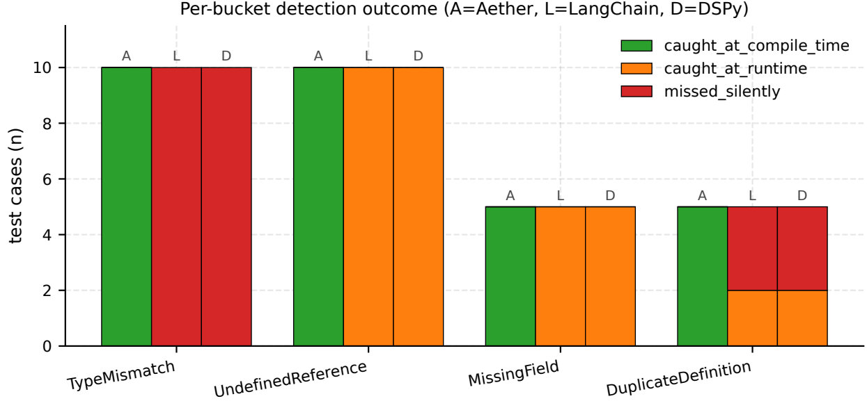
Figure 4: Type-safety bug-detection outcome by class ( n=10/10/5/5 ). Aether catches 30 cases at compile time; LangChain and DSPy catch 17 at runtime via Python exceptions and miss 13 silently. Methodology note: the original 'circular_dependency' bucket was substituted with 'duplicate_definition' due to a compiler pass-ordering gap ( SemanticError::CircularDependency is defined but preempted by other semantic-analysis errors) (full text in ablation_typesafety_v1.json#methodology_notes.cd_substitution ). Source: ablation_typesafety_v1.json .
