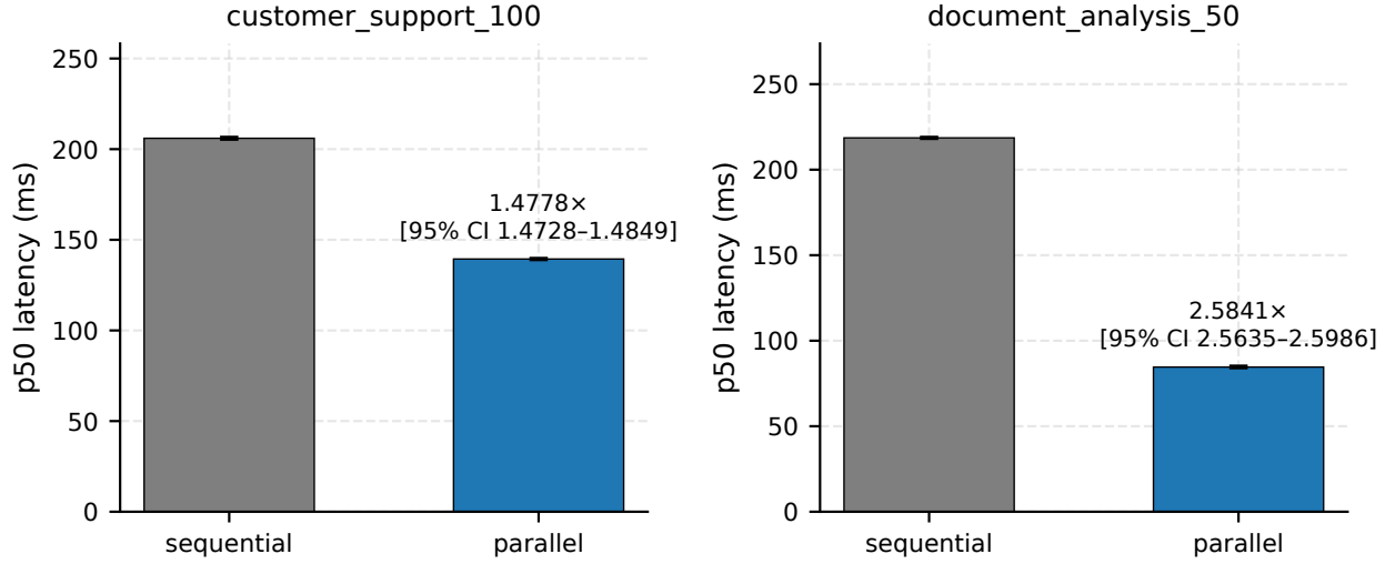
Figure 2: Sequential vs parallel p50 latency (ms) on the parallelization ablation. Speedup factors are paired BCa bootstrap with n_resamples=10000 , seed=42 (definition stored alongside the value in the source JSON). Source: ablation_parallel_v1.json .
