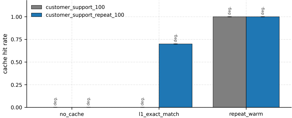
Figure 3: Cache hit rate by mode on the caching ablation. The unique-query workload ( customer_support_100 ) demonstrates L1’s null effect; the repeat-injected workload ( customer_support_repeat_100 ) demonstrates L1 effectiveness. Bars whose 95% CI collapses to a single value (per_trial values identical across all 5 trials) are labeled ‘(degenerate CI)’. Source: ablation_cache_v1.json .
