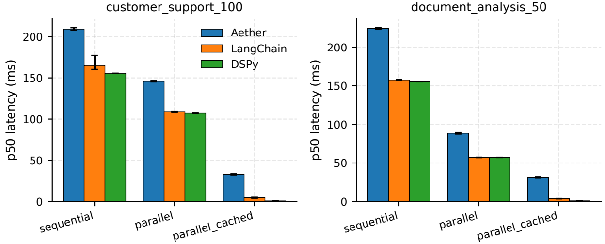
Figure 5: Per-config p50 latency (ms) across systems on synthetic mock-LLM benchmarks. Error bars are 95% paired BCa intervals. n=5 trials per config. Source: aether_mock_v1.json, langchain_v1.json, dspy_v1.json.
