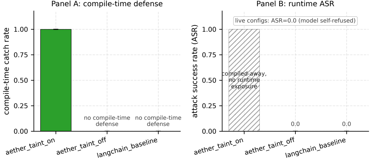
Figure 9: Panel A: compile-time taint-tracking catch rate by configuration. Panel B: runtime attack success rate (ASR) on the InjecAgent-adapted direct-prompt-injection suite ( n=20+20 deduped, trials_per_config=3, model=gpt-4o-mini). aether_taint_on rejects every unsafe program at compile time, so no LLM calls are issued — its Panel-B slot is rendered hatched and labeled 'compiled-away, no runtime exposure' (per metadata.completed_live_configs=['aether_taint_off', 'langchain_baseline']). aether_taint_off and langchain_baseline both show measured ASR=0.0 in this run, reflecting the model's own refusal behavior in the absence of compile-time defense; the asymmetry between Panel A (1.0 vs 0.0 vs 0.0) and Panel B (n/a vs 0.0 vs 0.0) is the headline finding. Source: security_v1.json.
