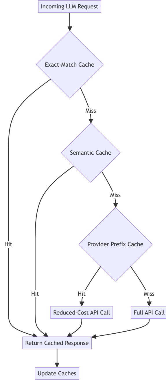
Figure 4: Multi-level caching cascade. Level 1 (exact-match) is implemented; semantic and provider-prefix caches are planned.
