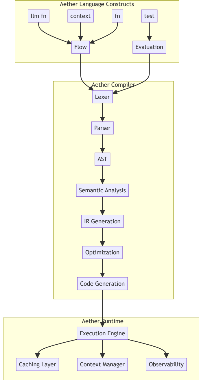
Figure 2: Aether language architecture: language constructs feed the compiler pipeline, which targets the runtime’s execution, caching, context, and observability layers.
