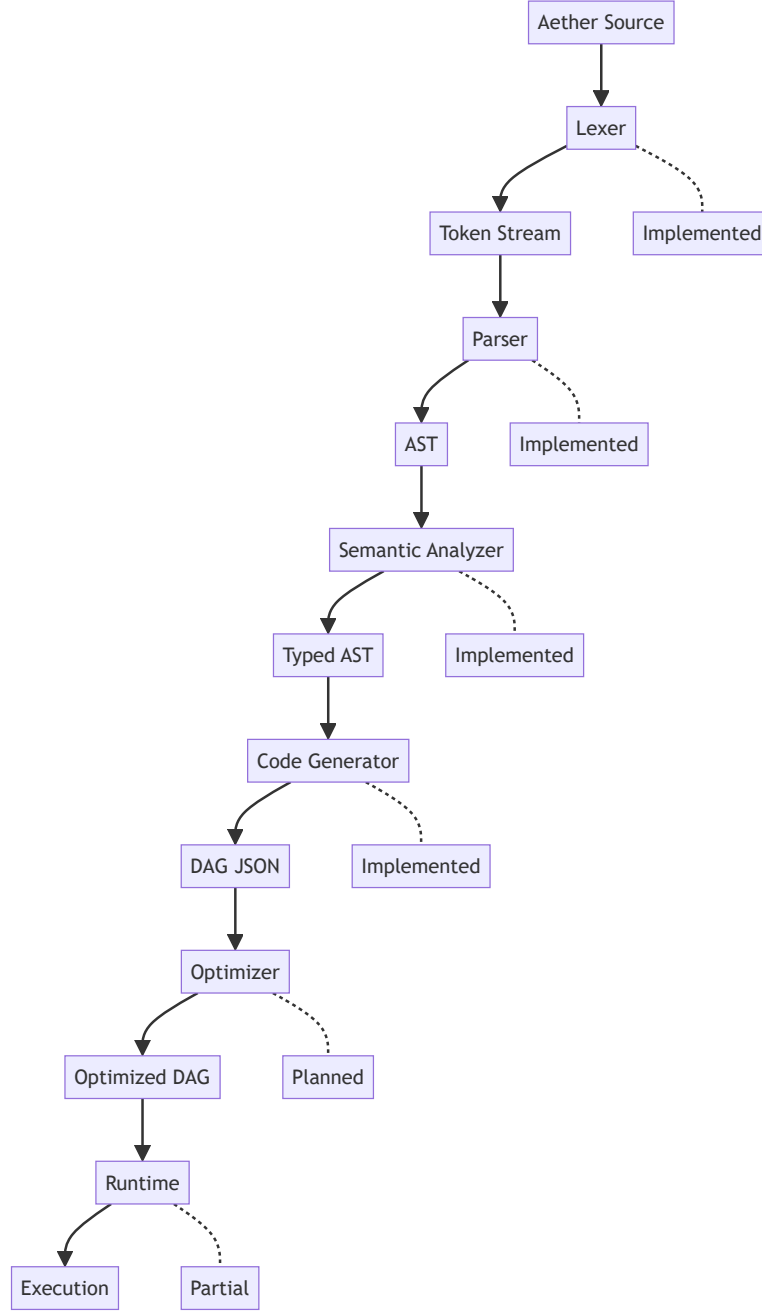
Figure 3: Aether compiler pipeline. Lexer, parser, semantic analyzer, and code generator are implemented; the optimizer is planned and the runtime is partial (see §6.2 for the status table).
