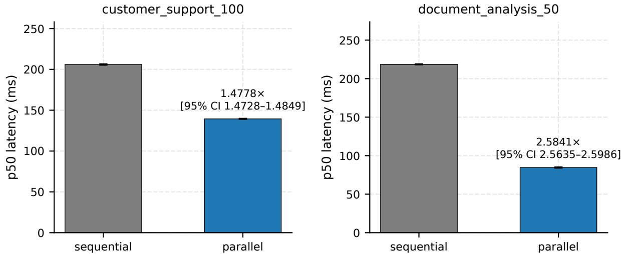
Figure 6: Sequential vs parallel p50 latency (ms) on the parallelization ablation. Speedup factors are paired BCa bootstrap with n\_resamples=10000 , seed=42 (definition stored alongside the value in the source JSON). Source: ablation_parallel_v1.json.
