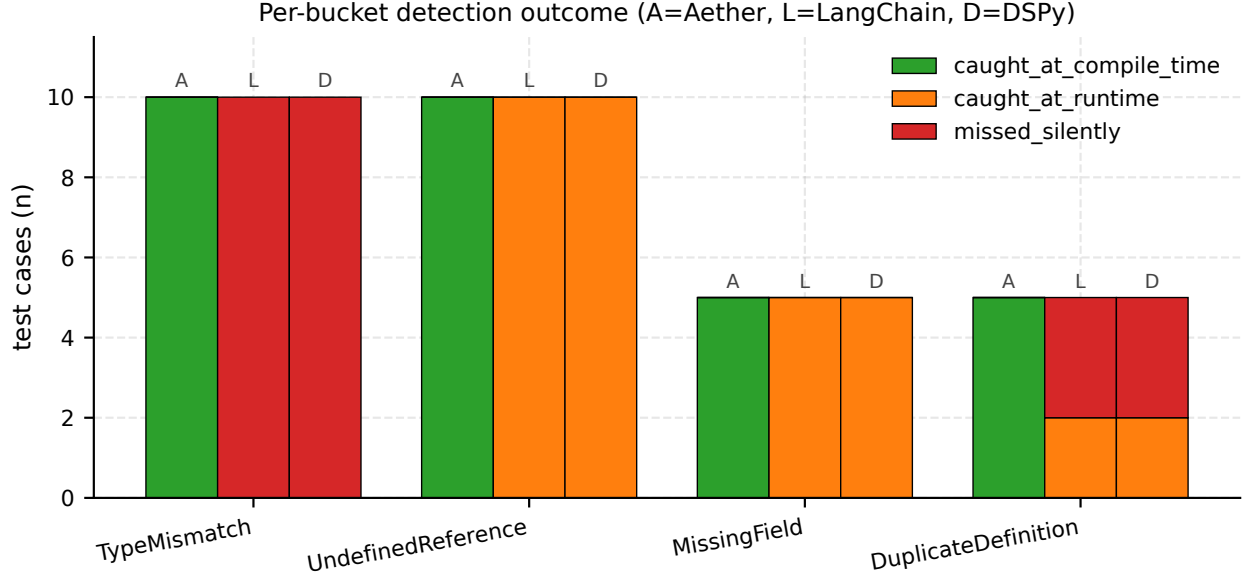
Figure 8: Type-safety bug-detection outcome by class (n=10/10/5/5). Aether catches 30 cases at compile time; LangChain and DSPy catch 17 at runtime via Python exceptions and miss 13 silently. Methodology note: the original 'circular_dependency' bucket was substituted with 'duplicate_definition' due to a compiler pass-ordering gap (SemanticError::CircularDependency is defined but preempted by other semantic-analysis errors) (full text in ablation_typesafety_v1.json#methodology_notes.cd_substitution ). Source: ablation_typesafety_v1.json .
