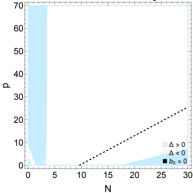
BY-model: Sign of \Delta for N_g = 4
