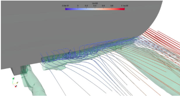
(a) Escala modelo, Fr = 0.16
