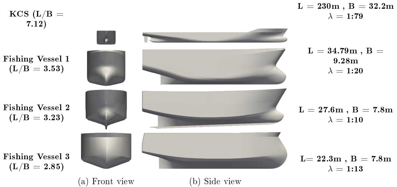
Figura 4.6.4: Tested models. The four hulls are shown scaled to equal length for direct comparison.
