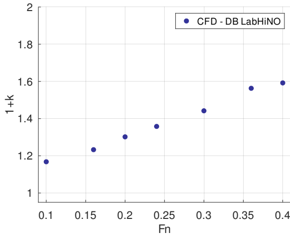
(a) Calado 1 (T1: 0.165 m)
