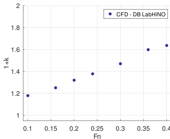
(c) Calado 3 (T3: 0.195 m)
