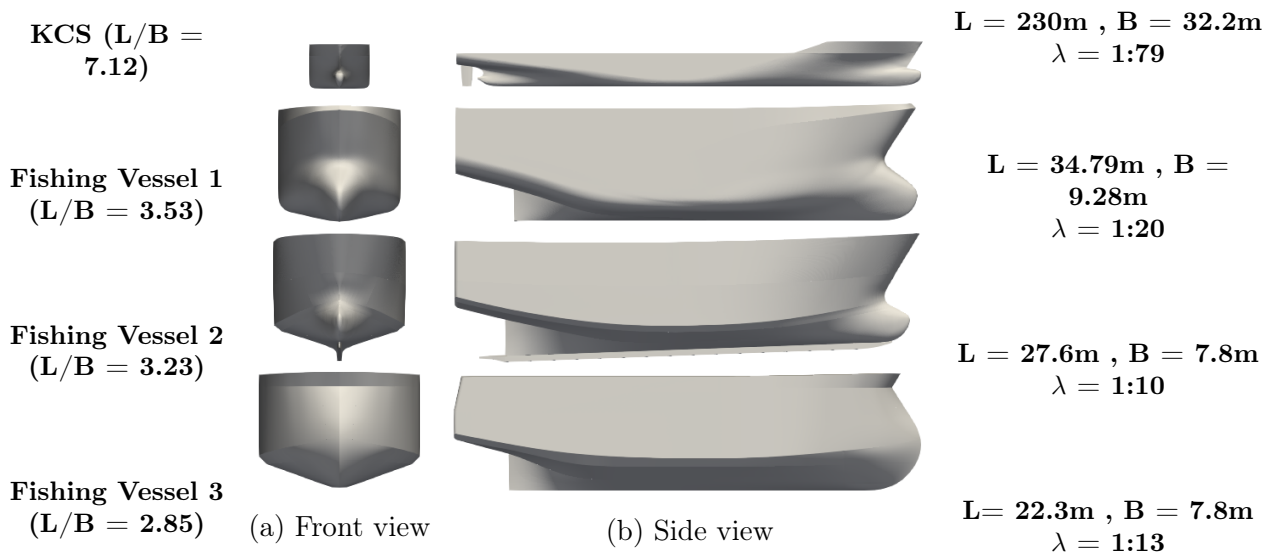
Figura 4.6.4: Tested models. The four hulls are shown scaled to equal length for direct comparison.
