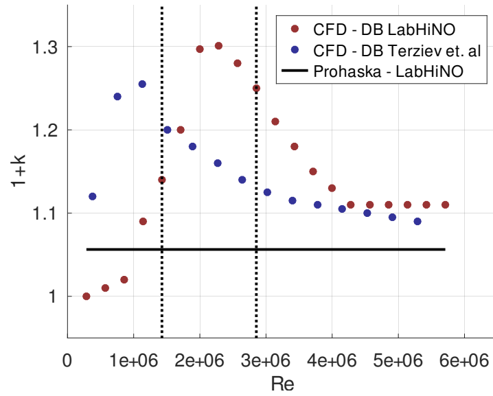
Figura 4.1.21: Numerical 1+k vs Re for the KCS 1:79 and 1:75 of Terziev et al. Terziev et al. [2021] .
