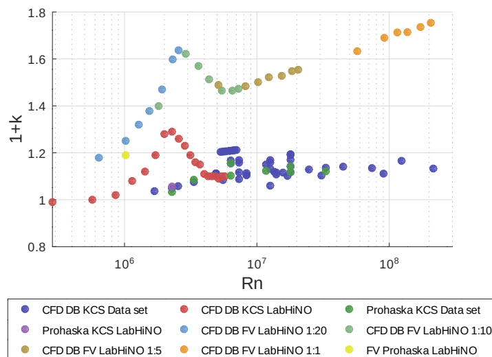
Figura 4.1.23: 1 + k vs Rn for the KCS and the fishing vessel (FV). KCS numerical (CFD DB) and experimental results (EFD) from present work and from Terziev et al. Data set Terziev et al. [2020]. Fishing vessel numerical (CFD DB, considering different scales) and experimental results (EFD) from present work. Logarithmic scale.
