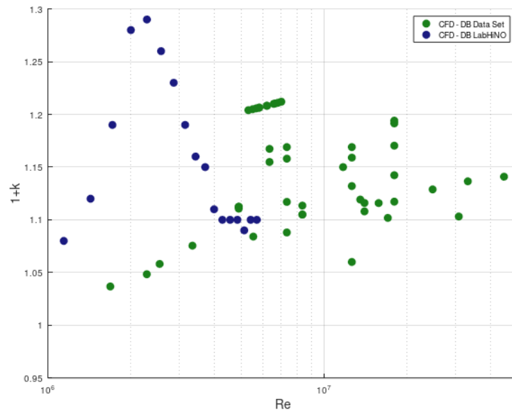
Figura 4.1.22: 1+k vs Re for the KCS. Numerical (CFD DB) results from present work and from Terziev et al. Data set [Terziev et al., 2020] .
