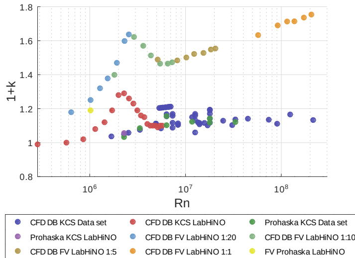
Figura 4.1.22: 1 + k vs Rn for the KCS and the fishing vessel (FV). KCS numerical (CFD DB) and experimental results (EFD) from present work and from Terziev et al. Data set Terziev et al. [2020]. Fishing vessel numerical (CFD DB, considering different scales) and experimental results (EFD) from present work. Logarithmic scale.
