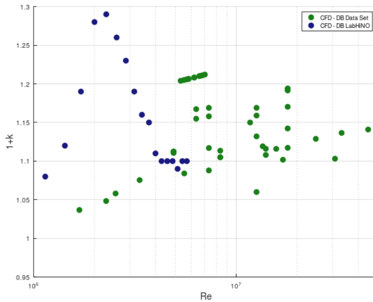
Figura 4.1.21: 1 + k vs Re for the KCS. Numerical (CFD DB) results from present work and from Terziev et al. Data set [Terziev et al., 2020] .
