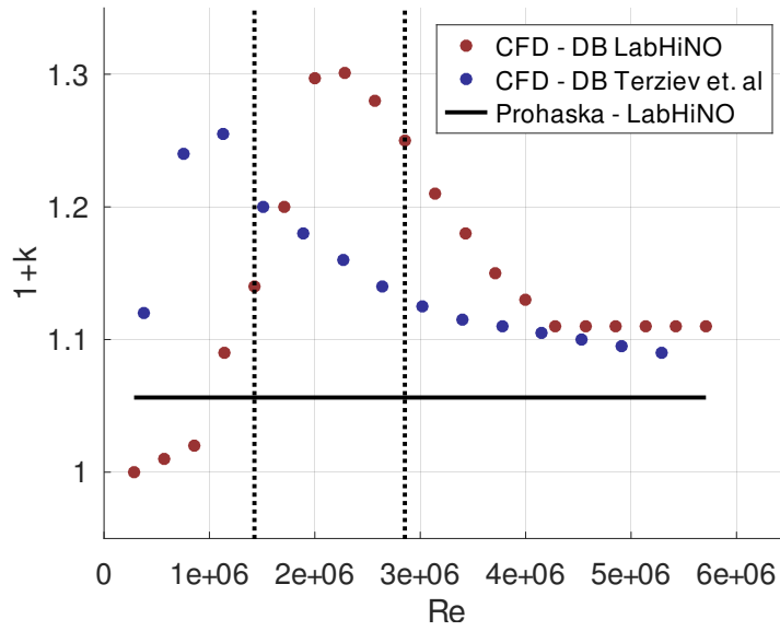
Figura 4.1.20: Numerical 1 + k vs Re for the KCS 1:79 and 1:75 of Terziev et al. Terziev et al. [2021] .
