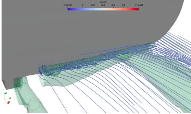
(c) Escala modelo, Fr = 0.36
