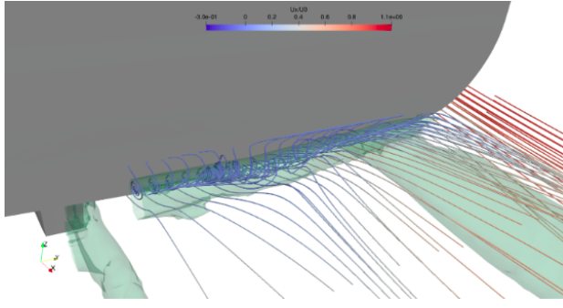
(a) Escala modelo, Fr = 0.16
