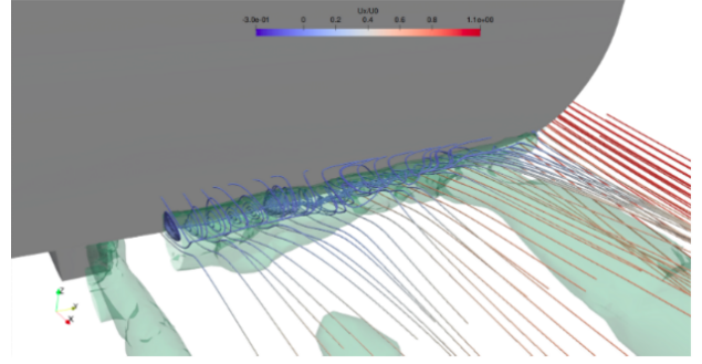
(b) Escala buque, Fr = 0.16
