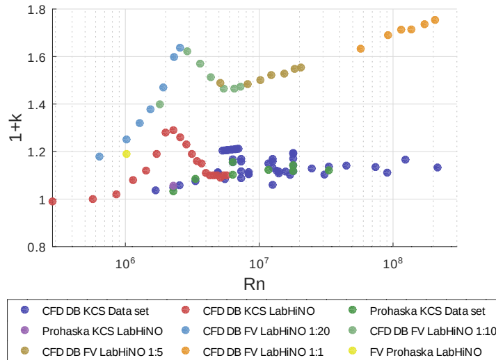
Figura 4.1.36: 1+k vs Rn for the KCS and the fishing vessel (FV). KCS numerical (CFD DB) and experimental results (EFD) from present work and from Terziev et al. Data set Terziev et al. [2020]. Fishing vessel numerical (CFD DB, considering different scales) and experimental results (EFD) from present work. Logarithmic scale.
