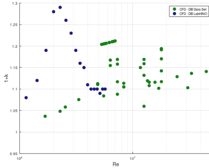
Figura 4.1.23: 1 + k vs Re for the KCS. Numerical (CFD DB) results from present work and from Terziev et al. Data set [Terziev et al., 2020].
