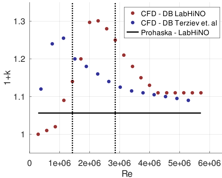
Figura 4.1.22: Numerical 1+k vs Re for the KCS 1:79 and 1:75 of Terziev et al. [Terziev et al., 2021].
