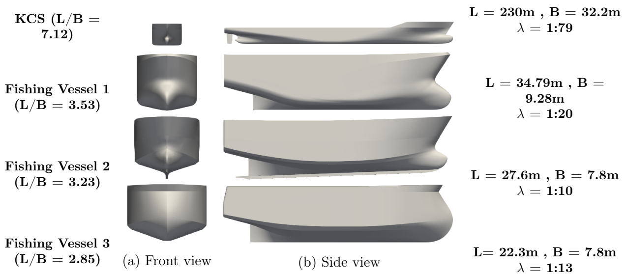
Figura 4.6.3: Tested models. The four hulls are shown scaled to equal length for direct comparison.
