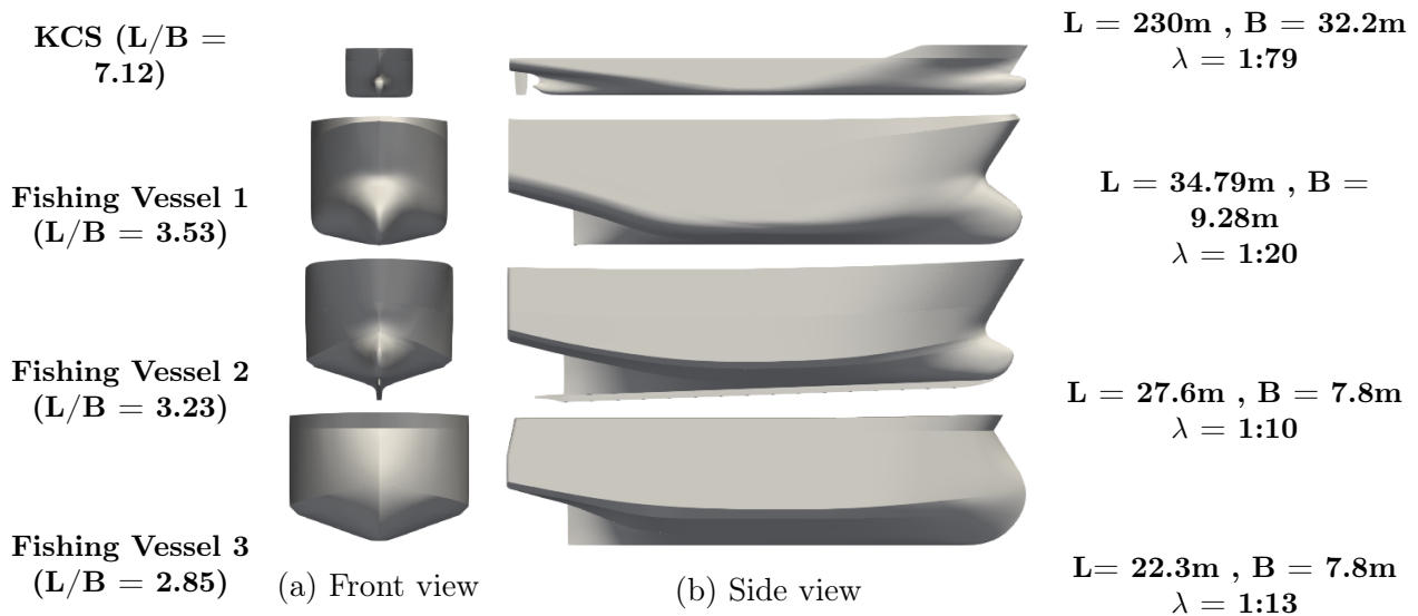
Figura 4.6.3: Tested models. The four hulls are shown scaled to equal length for direct comparison.
