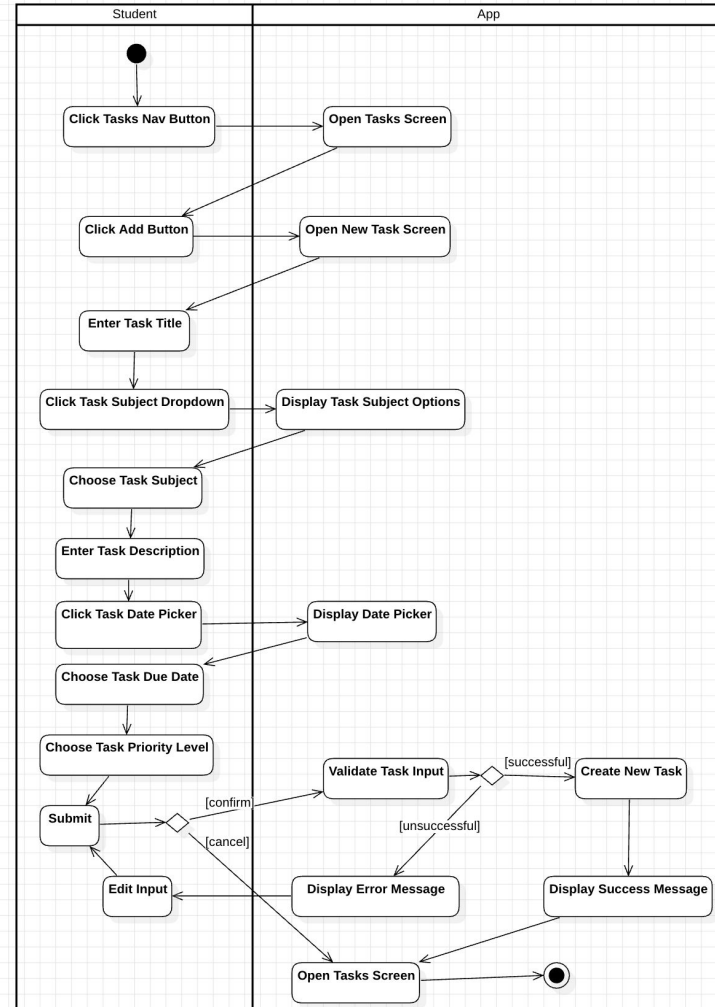
Create New Task Activity Diagram
