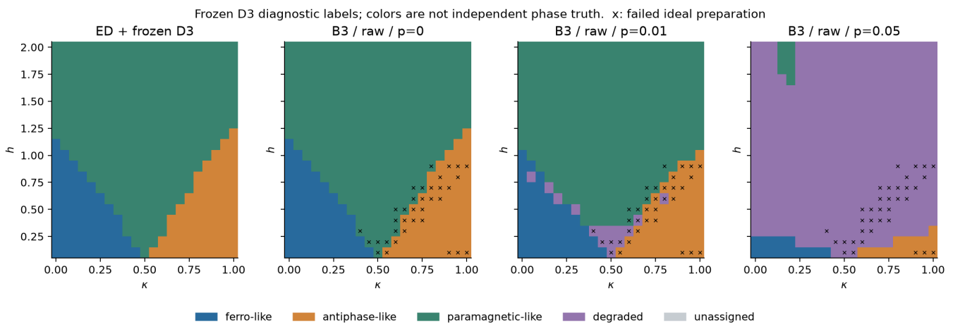
Figure 1. N8 PBC, h>0 . ED and three raw B3 noise levels share frozen D3 and color scale. Colors are phase-like estimates. Crosses retain preparation failures; reference coverage is separately available in the notebook.
