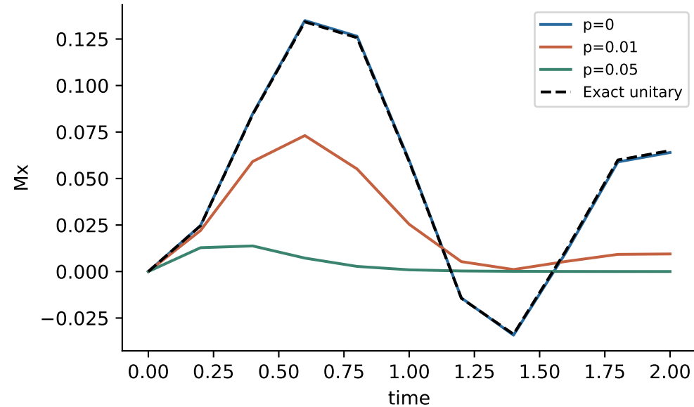
Archived dynamics control: kappa=.8, h=.8, zero product state, dt=.1 (not ground-state classification)
