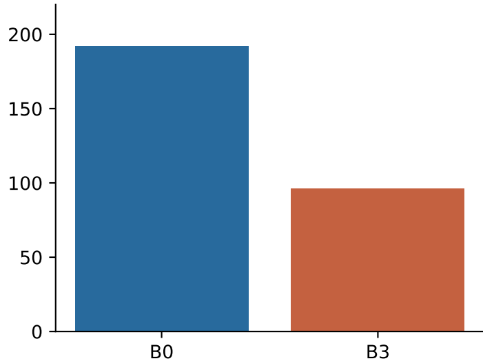
Median CNOTs
