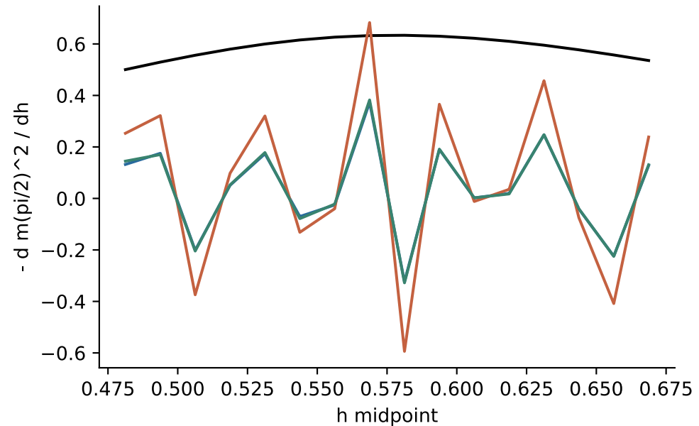
Fixed kappa=.8 window, p=.05: smaller errors need not restore a stable response peak
