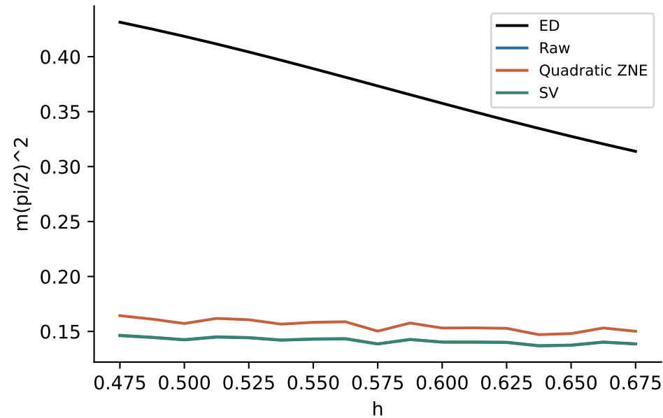
Fixed kappa=.8 window, p=.05: smaller errors need not restore a stable response peak
