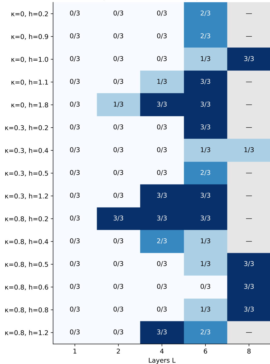
Joint passes / three runs; grey = not run
