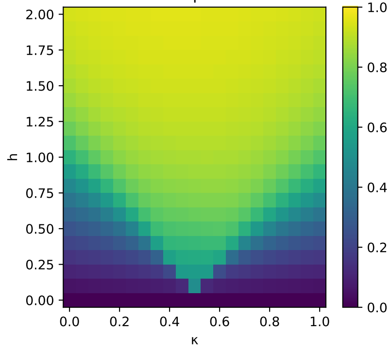
transverse polarization
