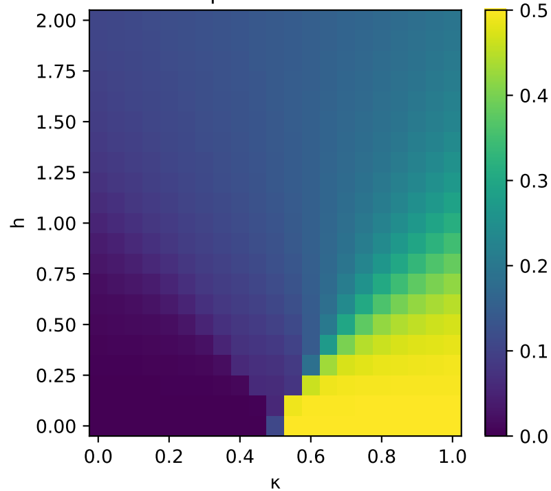
antiphase structure
