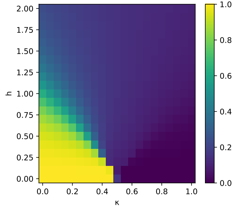
ferro structure
