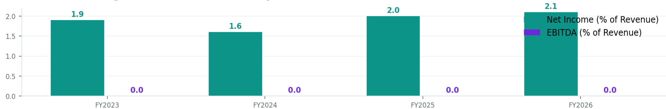
HDFCLIFE Margins as % of Revenue, by Year
